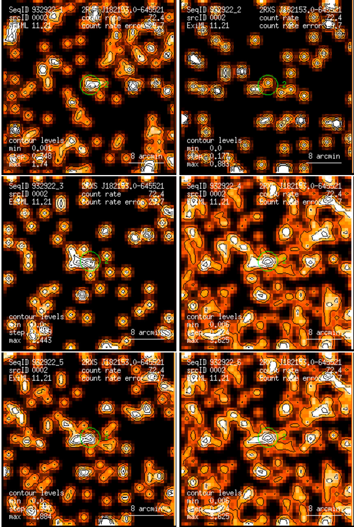
Figure 2: RASS 932922: detection 0002: band rate images, Gaussian filter: (1) PSPC channels 11 – 41, (2) 52 – 90, (3) 91 – 201, (4) 11 – 235, (5) 52 – 201, (6) 11 – 201. Broad band rates in counts/ks. Band rate contour levels in counts/ks/arcmin 2 .
