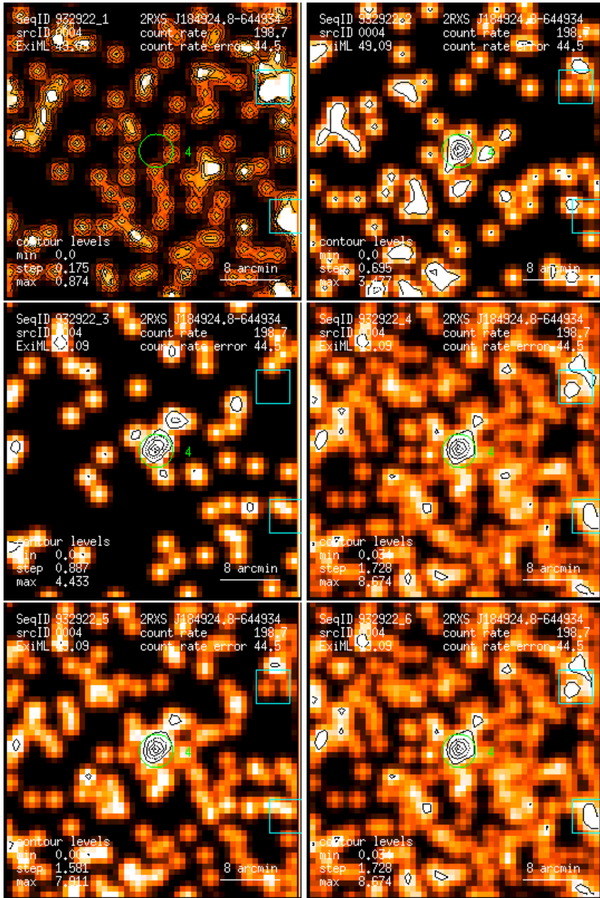
Figure 4: RASS 932922: detection 0004: band rate images, Gaussian filter: (1) PSPC channels 11 – 41, (2) 52 – 90, (3) 91 – 201, (4) 11 – 235, (5) 52 – 201, (6) 11 – 201. Broad band rates in counts/ks. Band rate contour levels in counts/ks/arcmin 2 .
