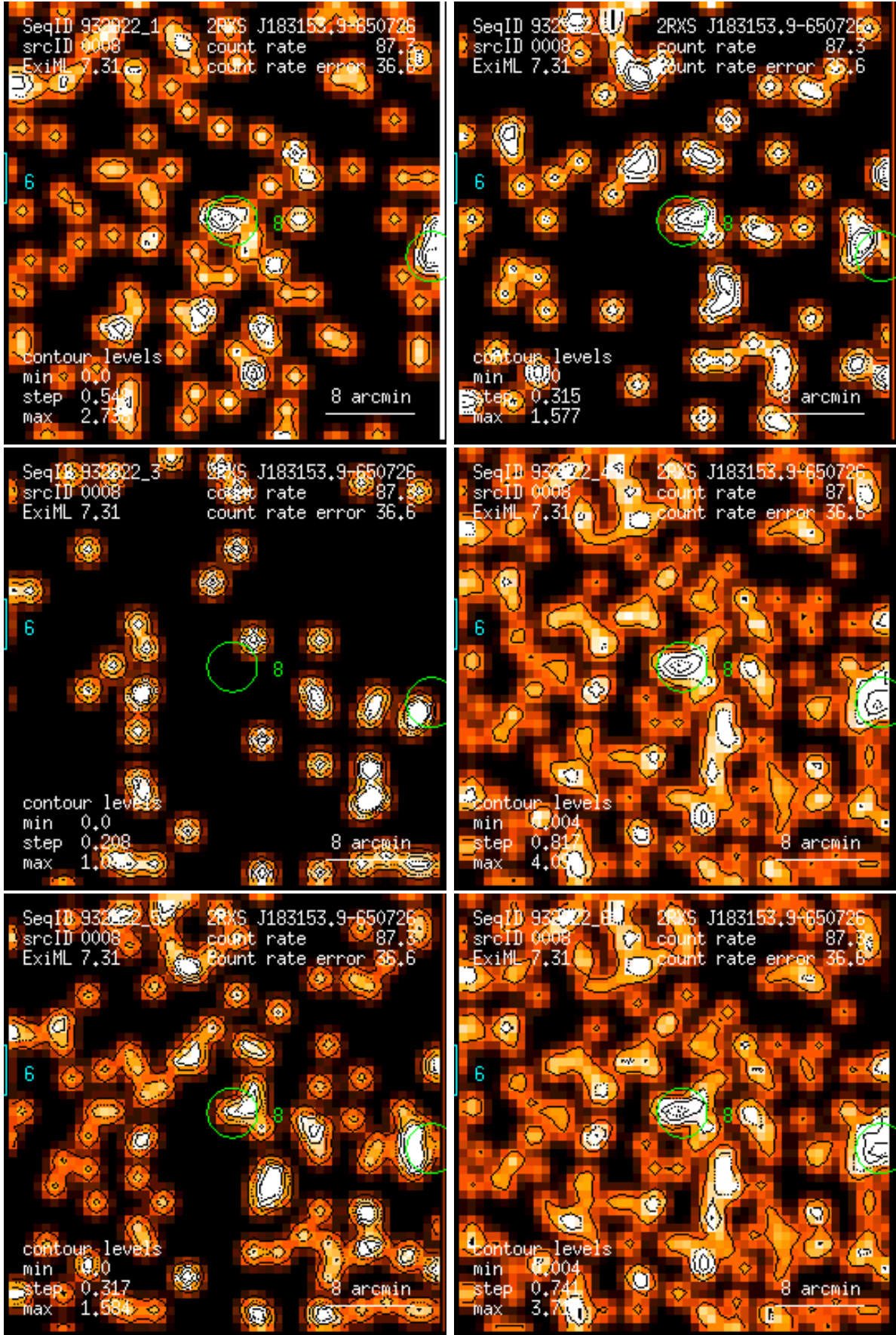
Figure 8: RASS 932922: detection 0008: band rate images, Gaussian filter: (1) PSPC channels 11 – 41, (2) 52 – 90, (3) 91 – 201, (4) 11 – 235, (5) 52 – 201, (6) 11 – 201. Broad band rates in counts/ks. Band rate contour levels in counts/ks/arcmin 2 .
