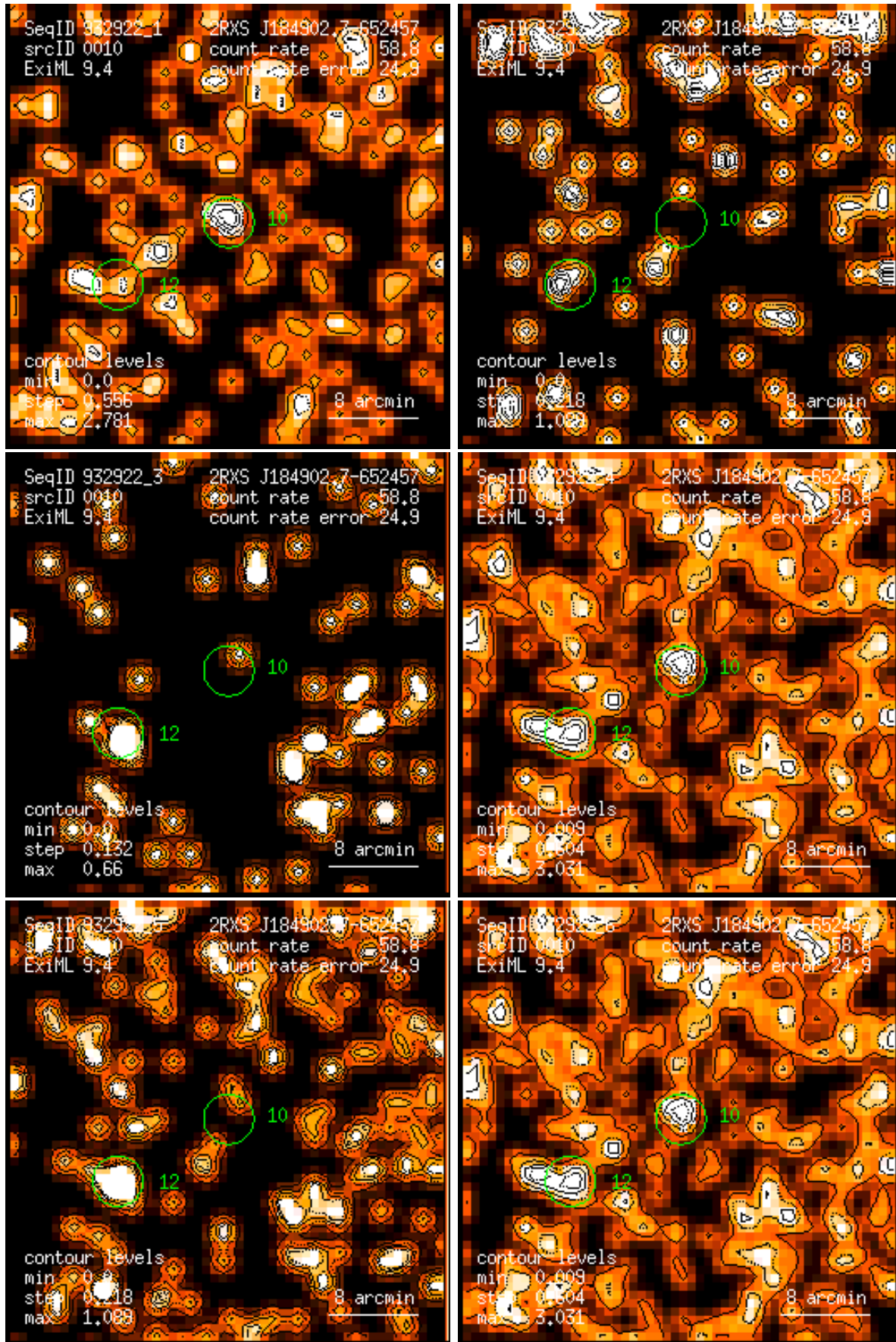
Figure 10: RASS 932922: detection 0010: band rate images, Gaussian filter: (1) PSPC channels 11 – 41, (2) 52 – 90, (3) 91 – 201, (4) 11 – 235, (5) 52 – 201, (6) 11 – 201. Broad band rates in counts/ks. Band rate contour levels in counts/ks/arcmin 2 .
