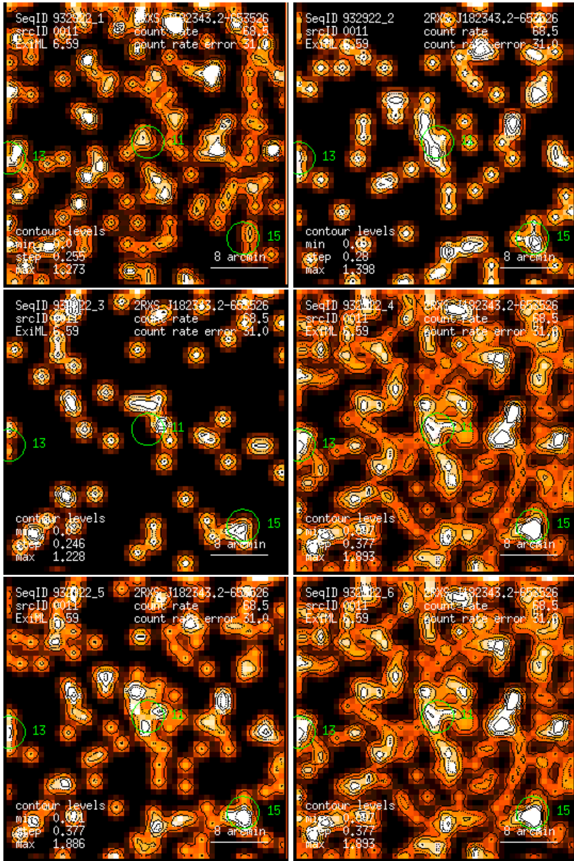
Figure 11: RASS 932922: detection 0011: band rate images, Gaussian filter: (1) PSPC channels 11 – 41, (2) 52 – 90, (3) 91 – 201, (4) 11 – 235, (5) 52 – 201, (6) 11 – 201. Broad band rates in counts/ks. Band rate contour levels in counts/ks/arcmin 2 .
