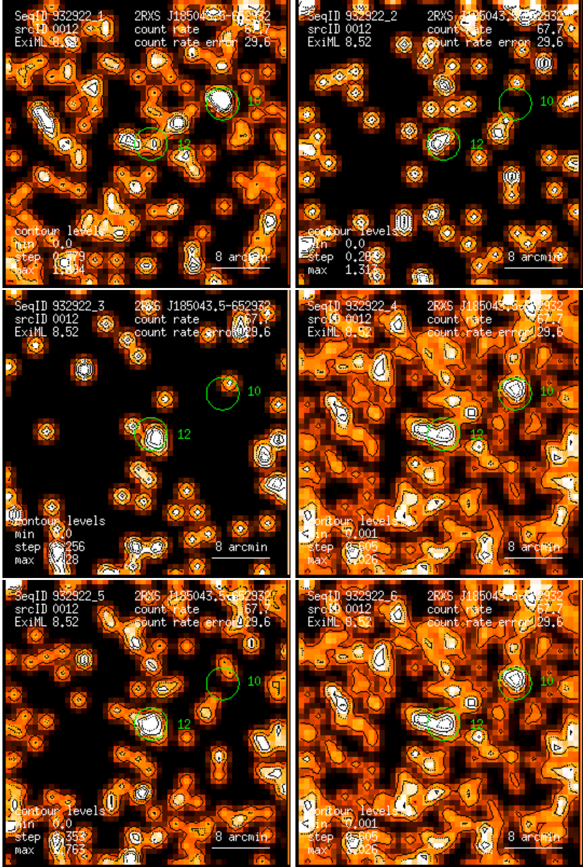
Figure 12: RASS 932922: detection 0012: band rate images, Gaussian filter: (1) PSPC channels 11 – 41, (2) 52 – 90, (3) 91 – 201, (4) 11 – 235, (5) 52 – 201, (6) 11 – 201. Broad band rates in counts/ks. Band rate contour levels in counts/ks/arcmin 2 .
