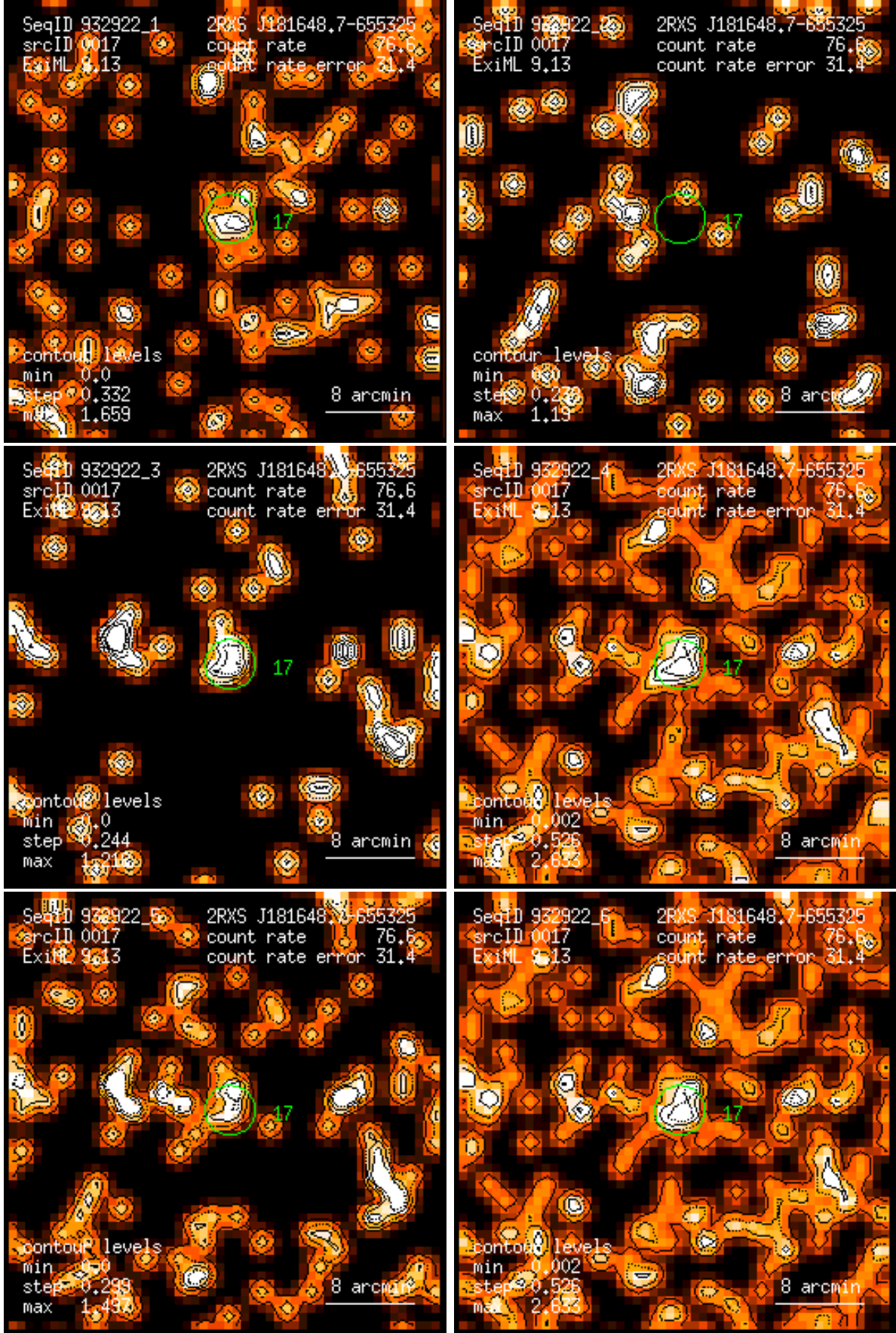
Figure 17: RASS 932922: detection 0017: band rate images, Gaussian filter: (1) PSPC channels 11 – 41, (2) 52 – 90, (3) 91 – 201, (4) 11 – 235, (5) 52 – 201, (6) 11 – 201. Broad band rates in counts/ks. Band rate contour levels in counts/ks/arcmin 2 .
