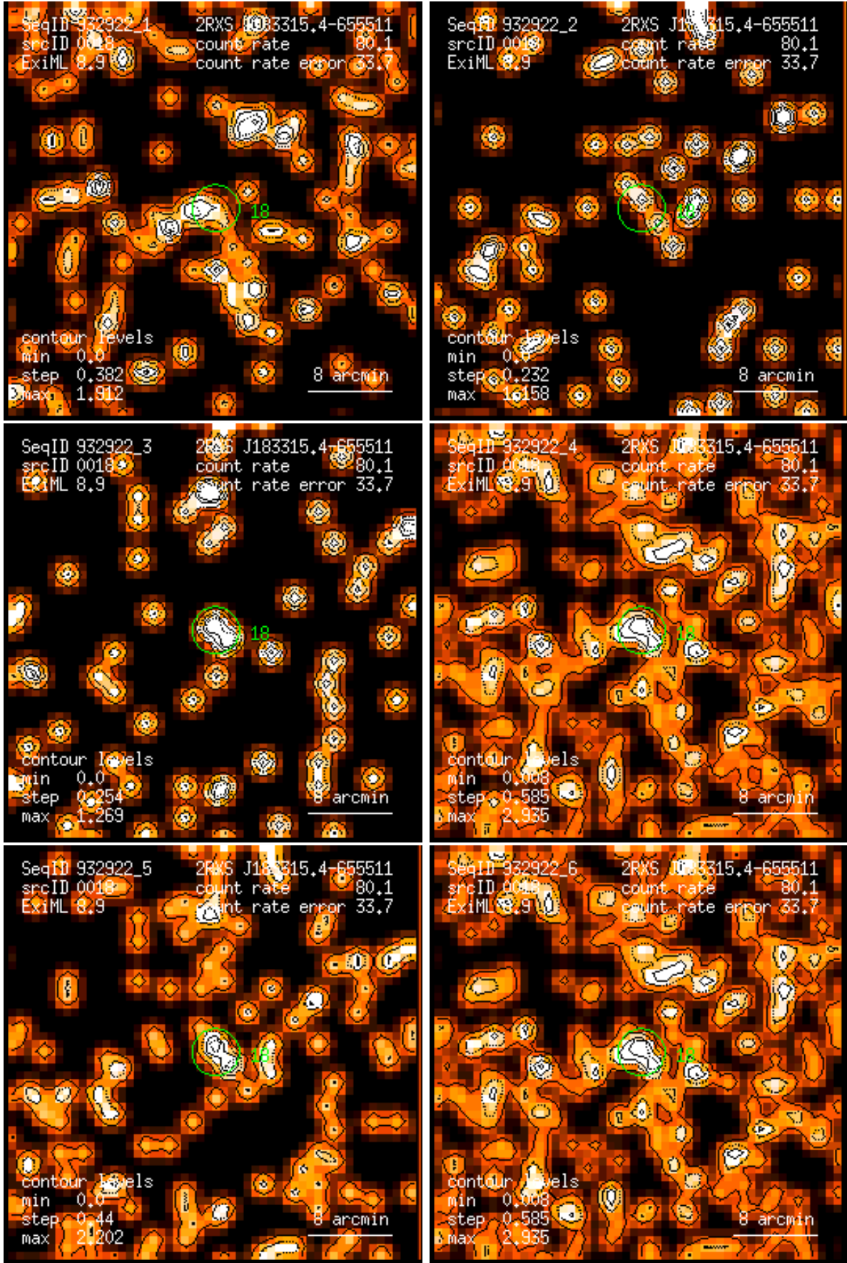
Figure 18: RASS 932922: detection 0018: band rate images, Gaussian filter: (1) PSPC channels 11 – 41, (2) 52 – 90, (3) 91 – 201, (4) 11 – 235, (5) 52 – 201, (6) 11 – 201. Broad band rates in counts/ks. Band rate contour levels in counts/ks/arcmin 2 .
