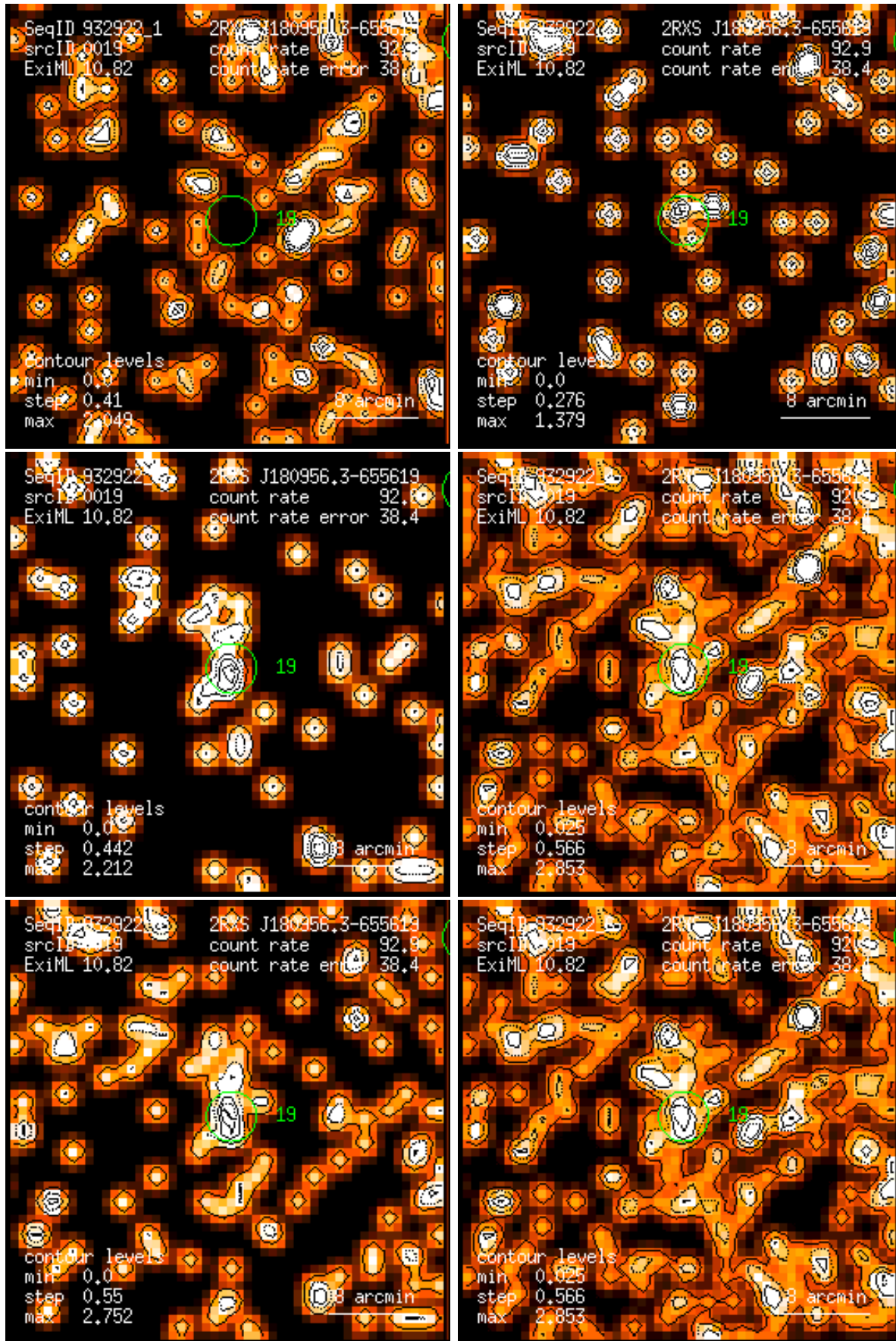
Figure 19: RASS 932922: detection 0019: band rate images, Gaussian filter: (1) PSPC channels 11 – 41, (2) 52 – 90, (3) 91 – 201, (4) 11 – 235, (5) 52 – 201, (6) 11 – 201. Broad band rates in counts/ks. Band rate contour levels in counts/ks/arcmin 2 .
