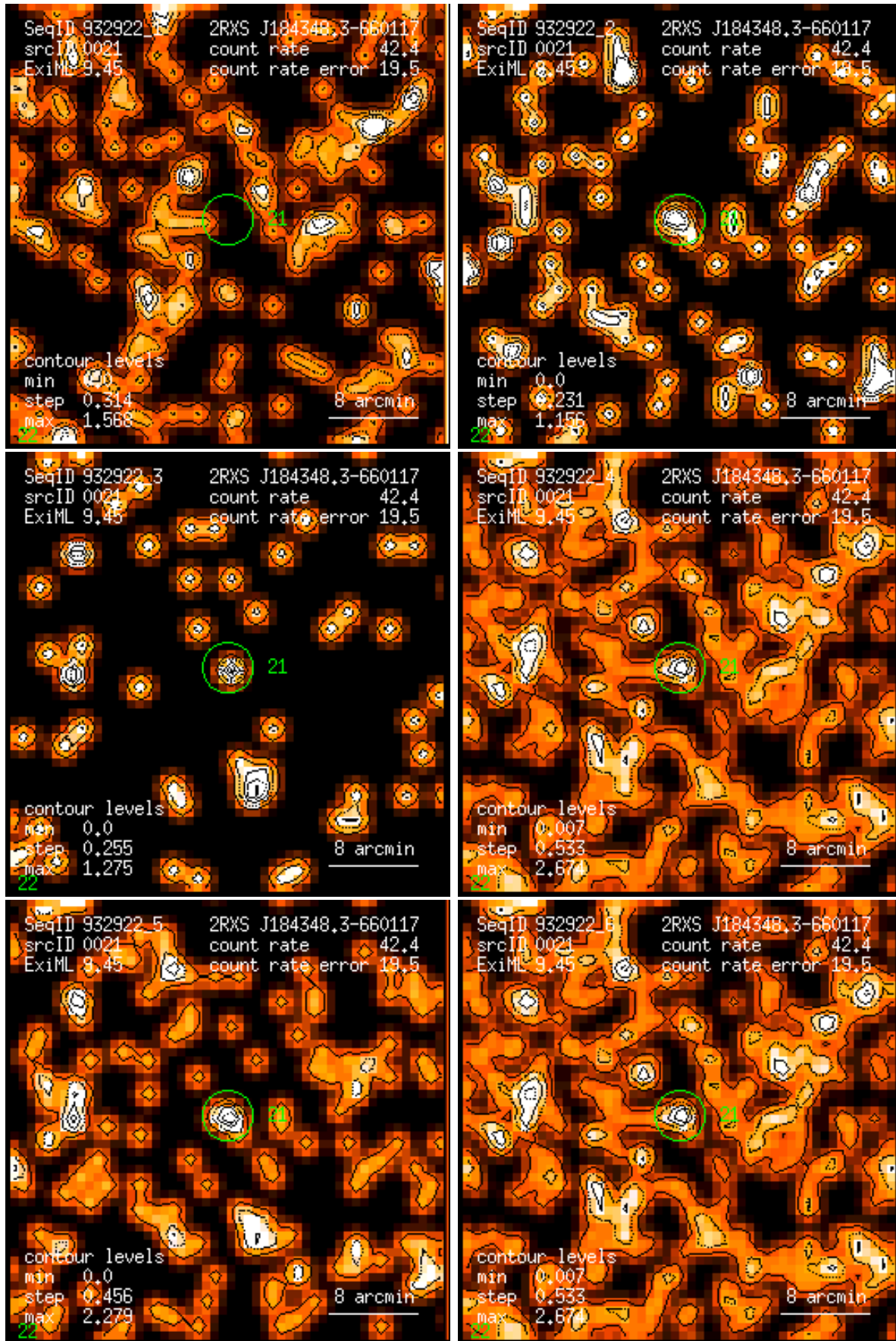
Figure 21: RASS 932922: detection 0021: band rate images, Gaussian filter: (1) PSPC channels 11 – 41, (2) 52 – 90, (3) 91 – 201, (4) 11 – 235, (5) 52 – 201, (6) 11 – 201. Broad band rates in counts/ks. Band rate contour levels in counts/ks/arcmin 2 .
