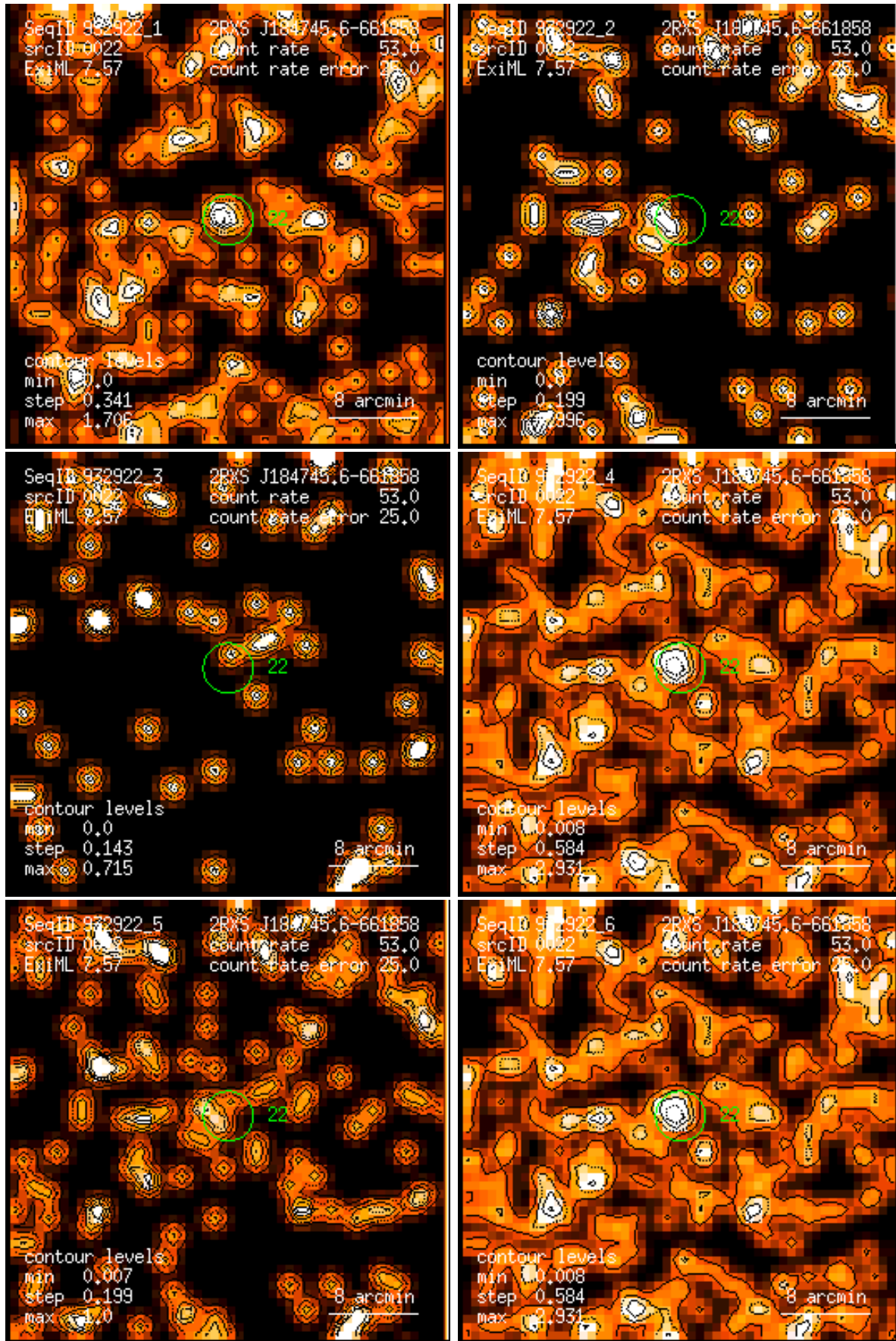
Figure 22: RASS 932922: detection 0022: band rate images, Gaussian filter: (1) PSPC channels 11 – 41, (2) 52 – 90, (3) 91 – 201, (4) 11 – 235, (5) 52 – 201, (6) 11 – 201. Broad band rates in counts/ks. Band rate contour levels in counts/ks/arcmin 2 .
