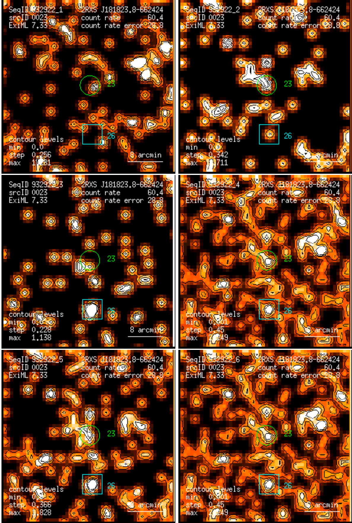
Figure 23: RASS 932922: detection 0023: band rate images, Gaussian filter: (1) PSPC channels 11 – 41, (2) 52 – 90, (3) 91 – 201, (4) 11 – 235, (5) 52 – 201, (6) 11 – 201. Broad band rates in counts/ks. Band rate contour levels in counts/ks/arcmin 2 .
