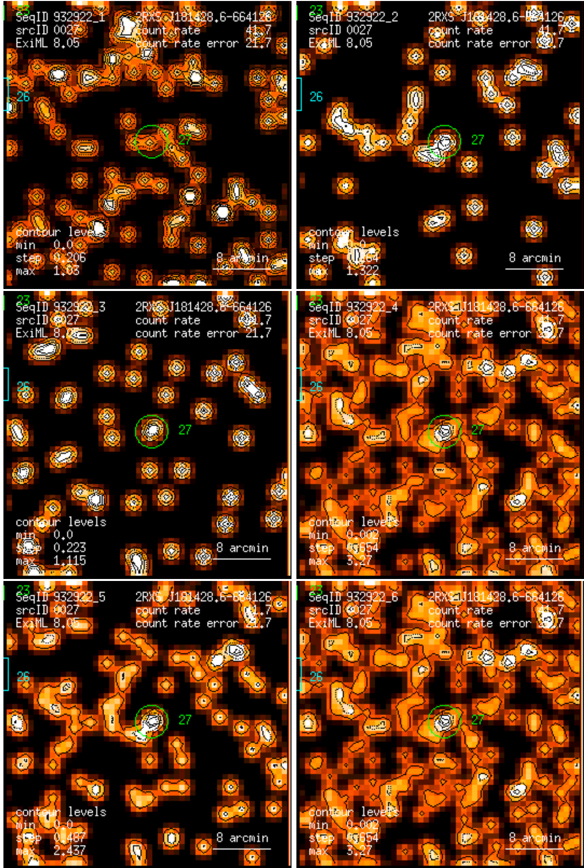
Figure 27: RASS 932922: detection 0027: band rate images, Gaussian filter: (1) PSPC channels 11 – 41, (2) 52 – 90, (3) 91 – 201, (4) 11 – 235, (5) 52 – 201, (6) 11 – 201. Broad band rates in counts/ks. Band rate contour levels in counts/ks/arcmin 2 .
