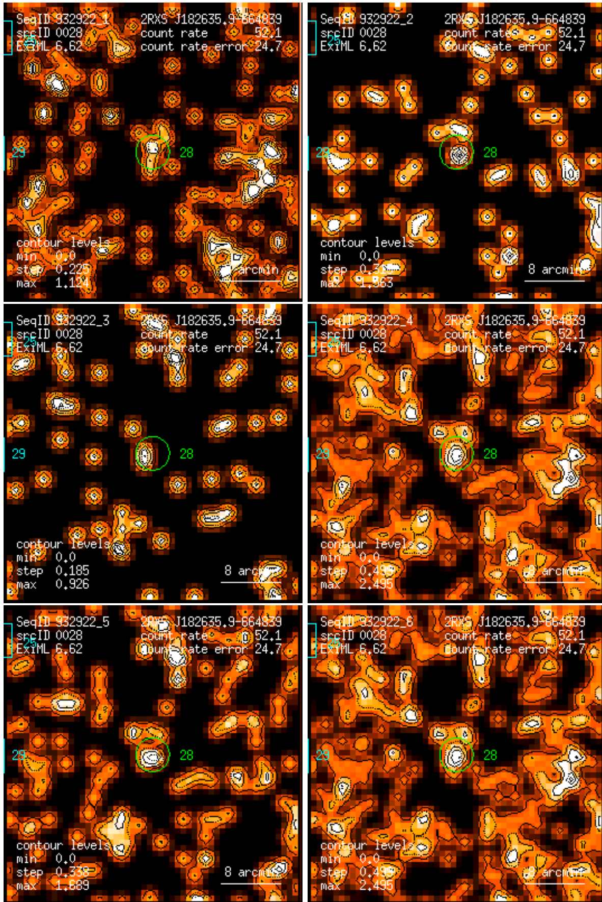
Figure 28: RASS 932922: detection 0028: band rate images, Gaussian filter: (1) PSPC channels 11 – 41, (2) 52 – 90, (3) 91 – 201, (4) 11 – 235, (5) 52 – 201, (6) 11 – 201. Broad band rates in counts/ks. Band rate contour levels in counts/ks/arcmin 2 .
