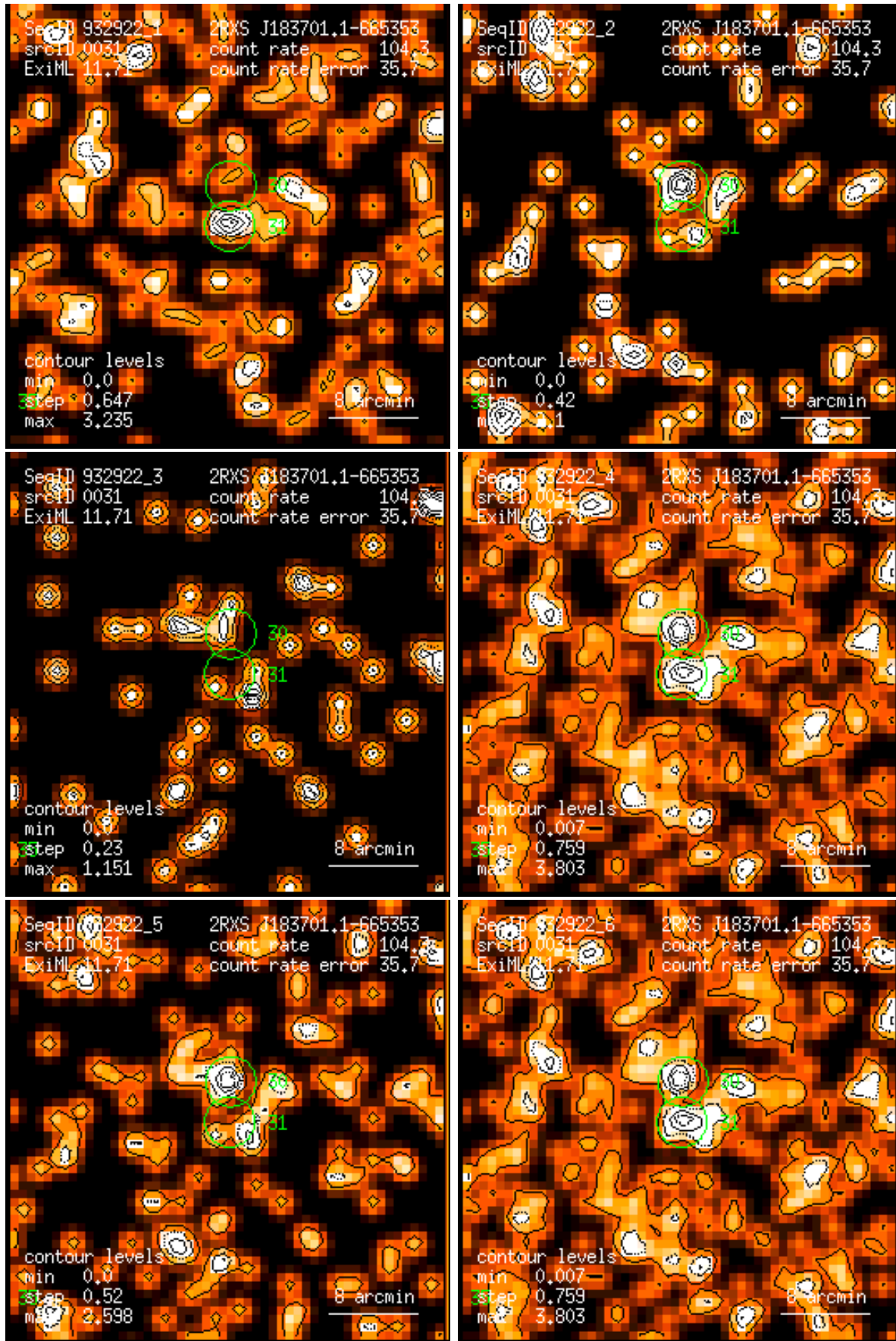
Figure 31: RASS 932922: detection 0031: band rate images, Gaussian filter: (1) PSPC channels 11 – 41, (2) 52 – 90, (3) 91 – 201, (4) 11 – 235, (5) 52 – 201, (6) 11 – 201. Broad band rates in counts/ks. Band rate contour levels in counts/ks/arcmin 2 .
