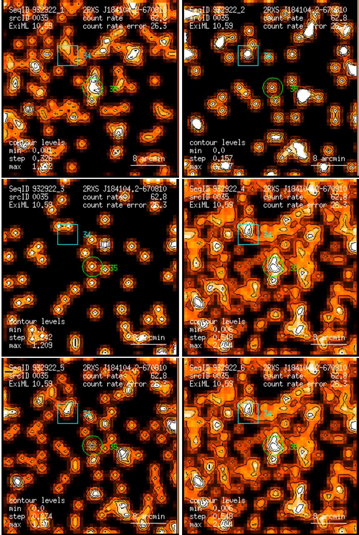
Figure 35: RASS 932922: detection 0035: band rate images, Gaussian filter: (1) PSPC channels 11 – 41, (2) 52 – 90, (3) 91 – 201, (4) 11 – 235, (5) 52 – 201, (6) 11 – 201. Broad band rates in counts/ks. Band rate contour levels in counts/ks/arcmin 2 .
