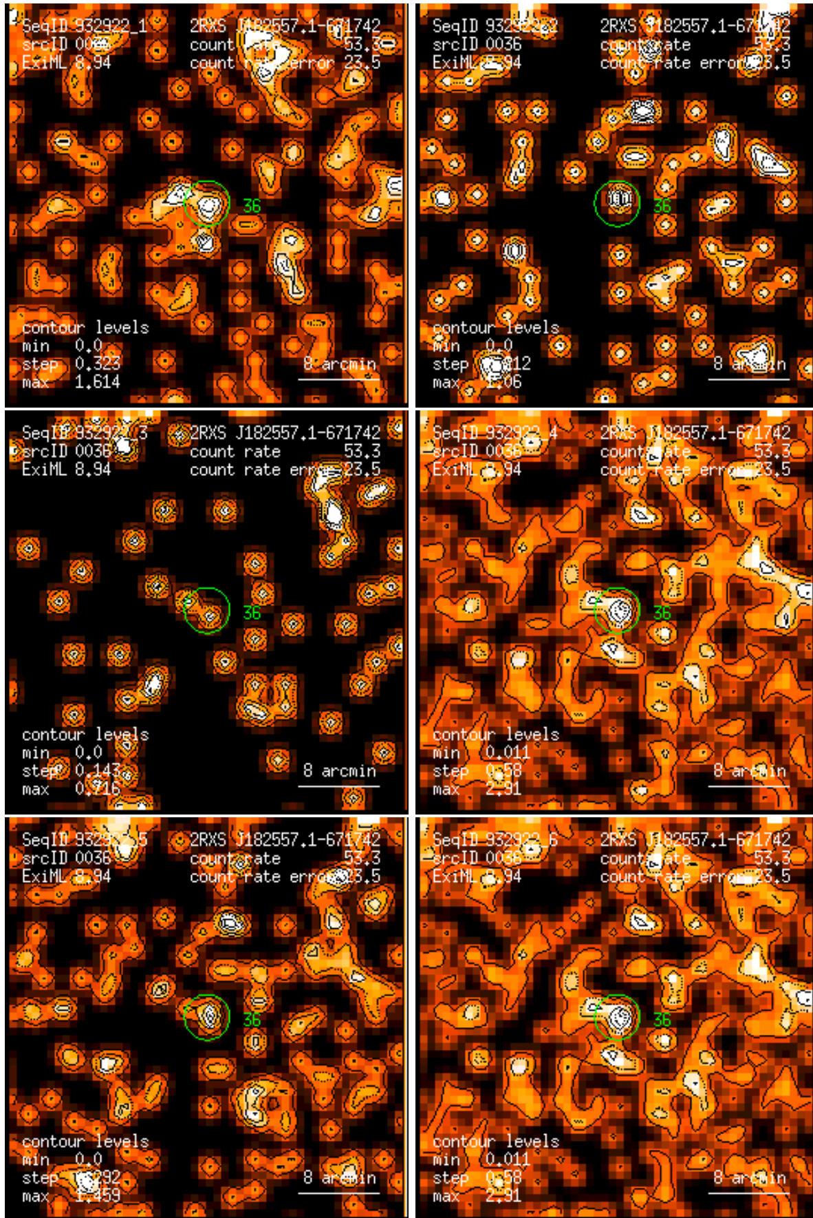
Figure 36: RASS 932922: detection 0036: band rate images, Gaussian filter: (1) PSPC channels 11 – 41, (2) 52 – 90, (3) 91 – 201, (4) 11 – 235, (5) 52 – 201, (6) 11 – 201. Broad band rates in counts/ks. Band rate contour levels in counts/ks/arcmin 2 .
