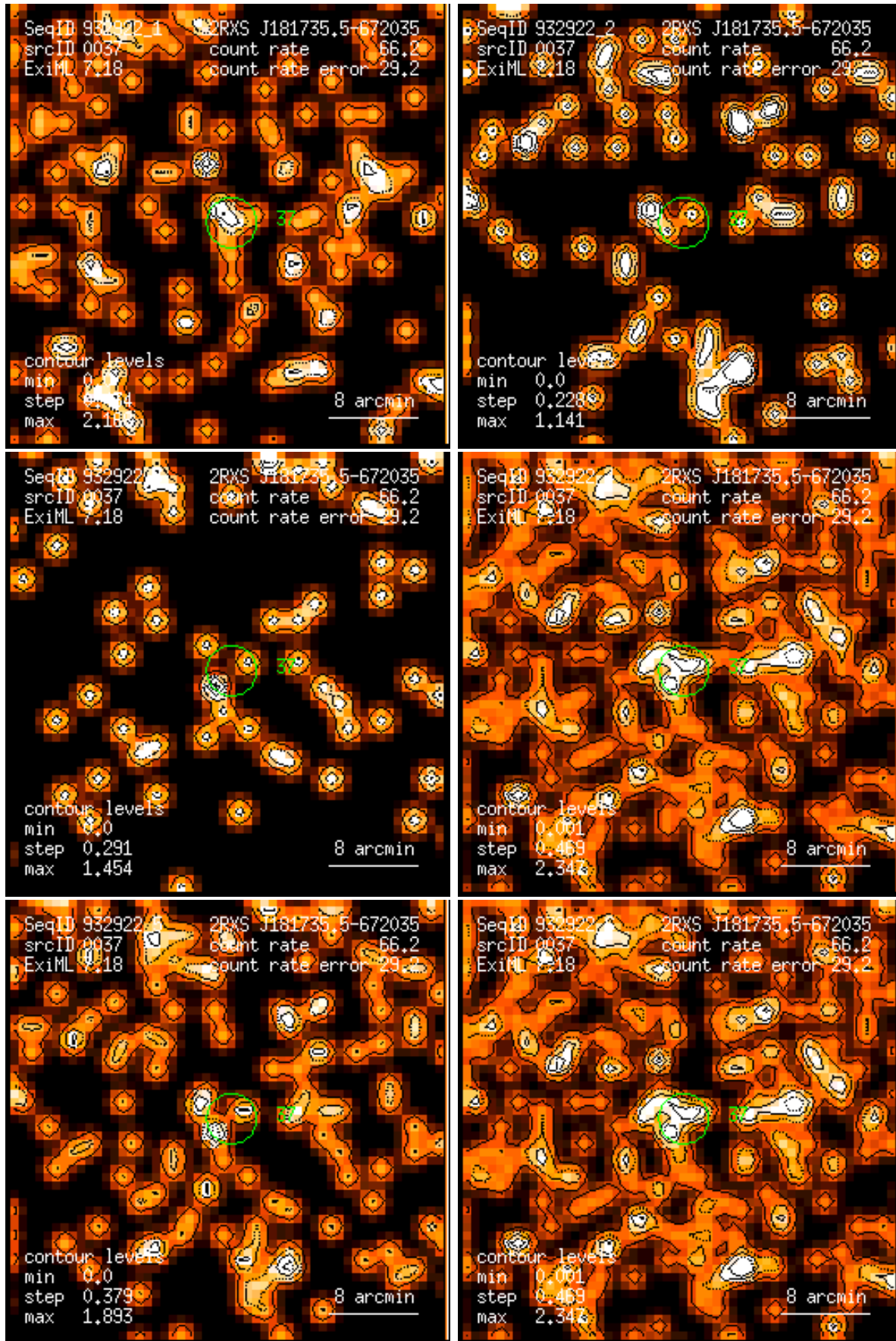
Figure 37: RASS 932922: detection 0037: band rate images, Gaussian filter: (1) PSPC channels 11 – 41, (2) 52 – 90, (3) 91 – 201, (4) 11 – 235, (5) 52 – 201, (6) 11 – 201. Broad band rates in counts/ks. Band rate contour levels in counts/ks/arcmin 2 .
