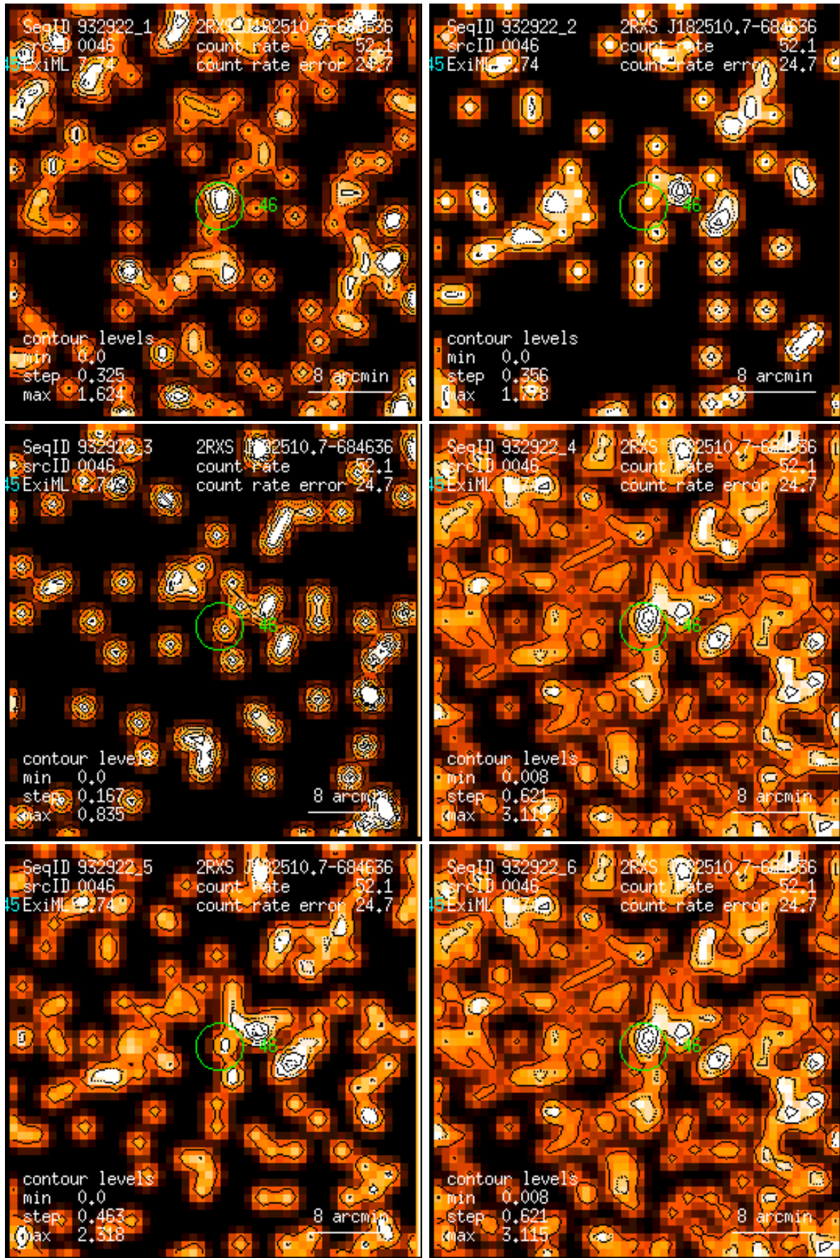
Figure 46: RASS 932922: detection 0046: band rate images, Gaussian filter: (1) PSPC channels 11 – 41, (2) 52 – 90, (3) 91 – 201, (4) 11 – 235, (5) 52 – 201, (6) 11 – 201. Broad band rates in counts/ks. Band rate contour levels in counts/ks/arcmin 2 .
