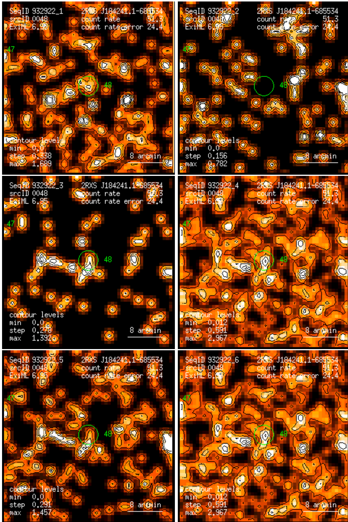
Figure 48: RASS 932922: detection 0048: band rate images, Gaussian filter: (1) PSPC channels 11 – 41, (2) 52 – 90, (3) 91 – 201, (4) 11 – 235, (5) 52 – 201, (6) 11 – 201. Broad band rates in counts/ks. Band rate contour levels in counts/ks/arcmin 2 .
