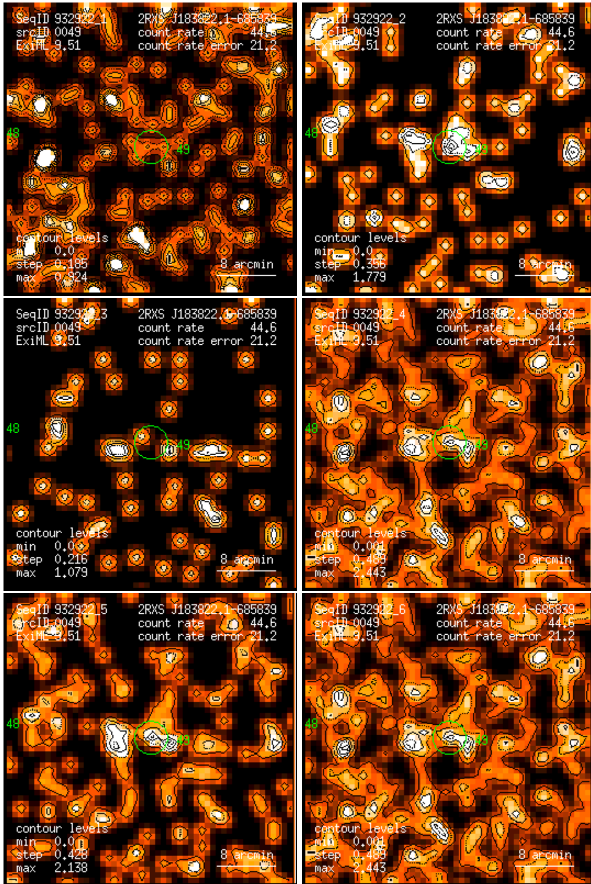
Figure 49: RASS 932922: detection 0049: band rate images, Gaussian filter: (1) PSPC channels 11 – 41, (2) 52 – 90, (3) 91 – 201, (4) 11 – 235, (5) 52 – 201, (6) 11 – 201. Broad band rates in counts/ks. Band rate contour levels in counts/ks/arcmin 2 .
