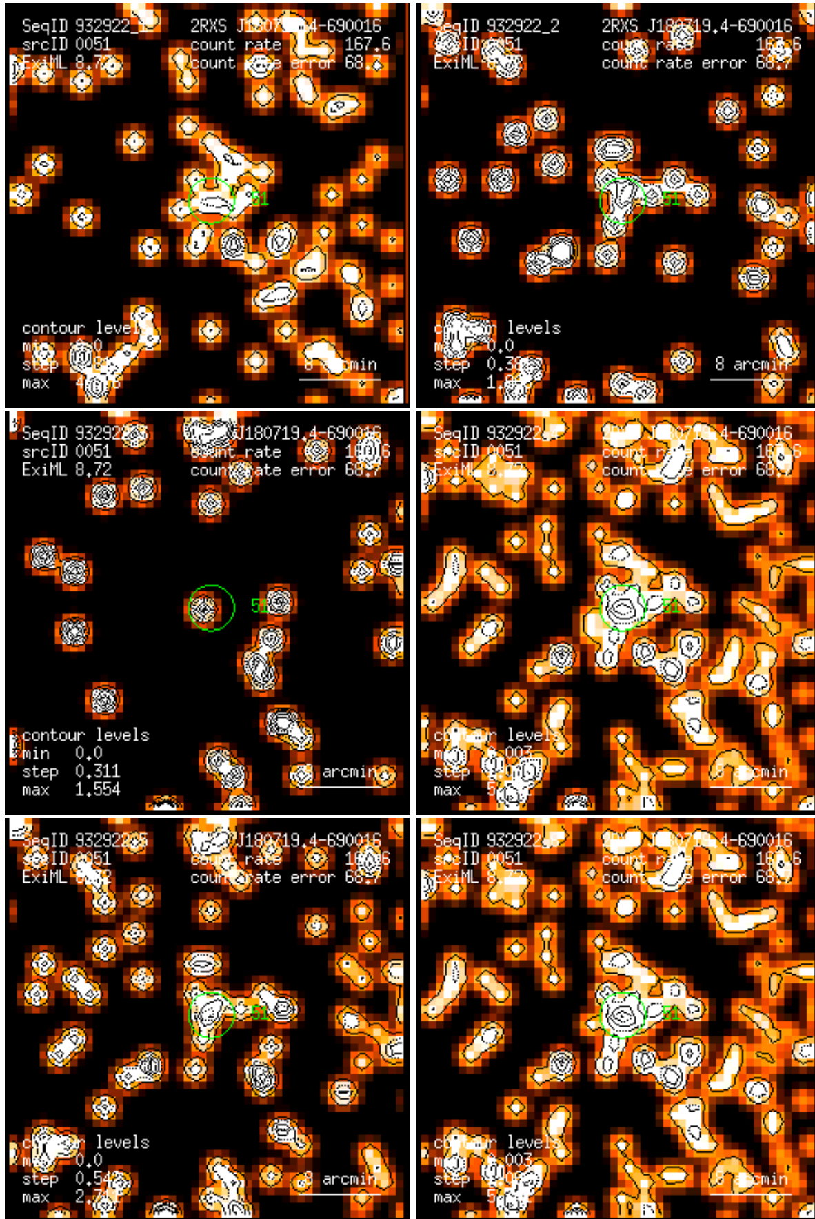
Figure 51: RASS 932922: detection 0051: band rate images, Gaussian filter: (1) PSPC channels 11 – 41, (2) 52 – 90, (3) 91 – 201, (4) 11 – 235, (5) 52 – 201, (6) 11 – 201. Broad band rates in counts/ks. Band rate contour levels in counts/ks/arcmin 2 .
