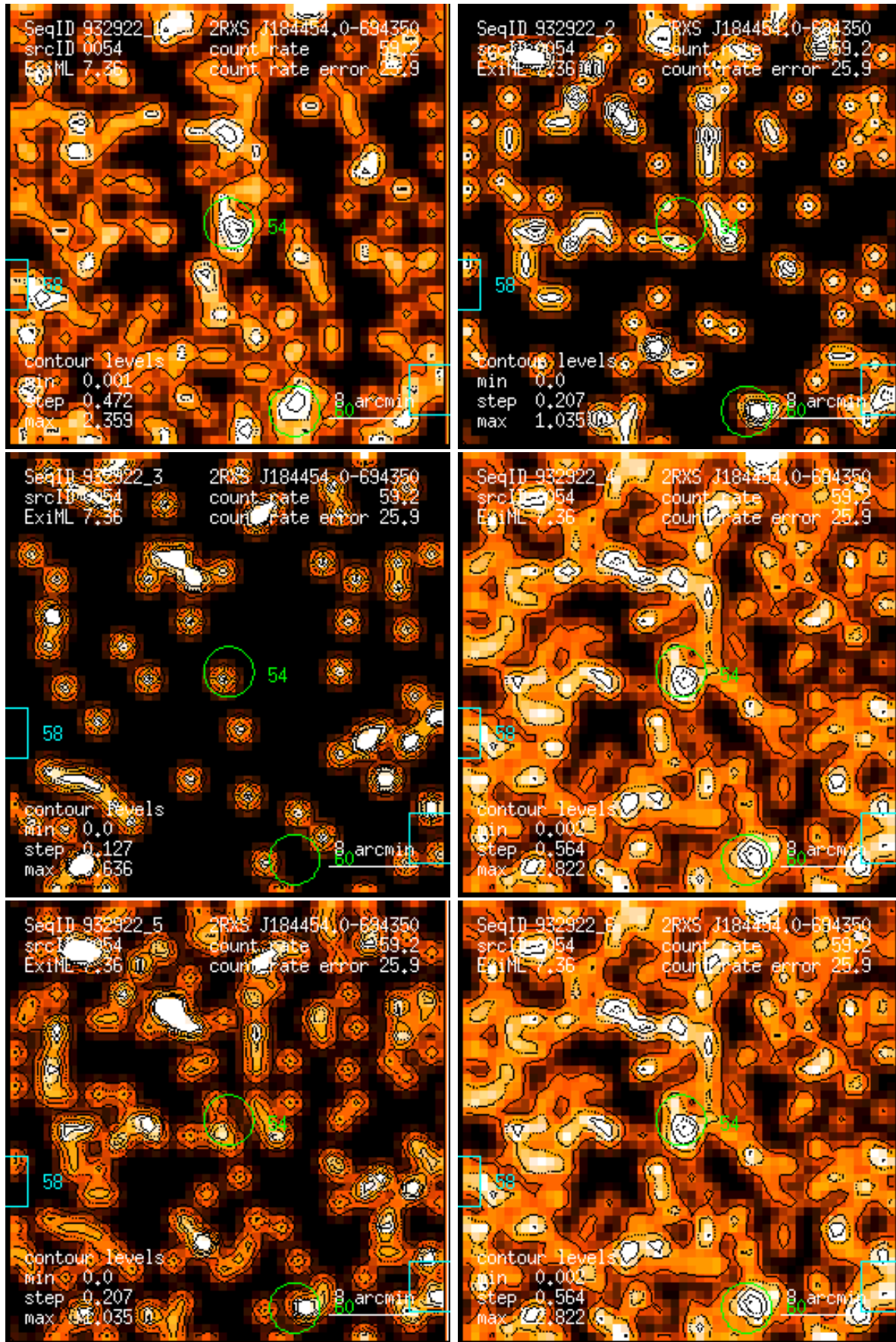
Figure 54: RASS 932922: detection 0054: band rate images, Gaussian filter: (1) PSPC channels 11 – 41, (2) 52 – 90, (3) 91 – 201, (4) 11 – 235, (5) 52 – 201, (6) 11 – 201. Broad band rates in counts/ks. Band rate contour levels in counts/ks/arcmin 2 .
