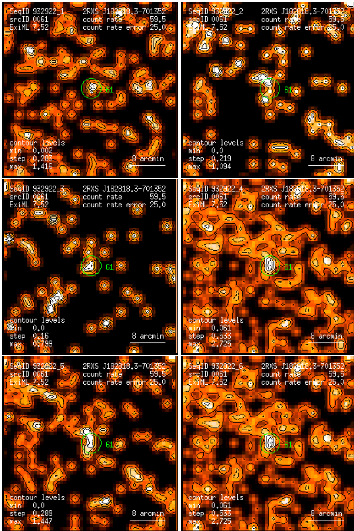
Figure 61: RASS 932922: detection 0061: band rate images, Gaussian filter: (1) PSPC channels 11 – 41, (2) 52 – 90, (3) 91 – 201, (4) 11 – 235, (5) 52 – 201, (6) 11 – 201. Broad band rates in counts/ks. Band rate contour levels in counts/ks/arcmin 2 .
