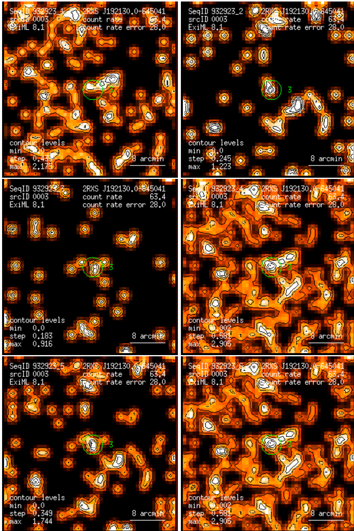
Figure 3: RASS 932923: detection 0003: band rate images, Gaussian filter: (1) PSPC channels 11 – 41, (2) 52 – 90, (3) 91 – 201, (4) 11 – 235, (5) 52 – 201, (6) 11 – 201. Broad band rates in counts/ks. Band rate contour levels in counts/ks/arcmin 2 .
