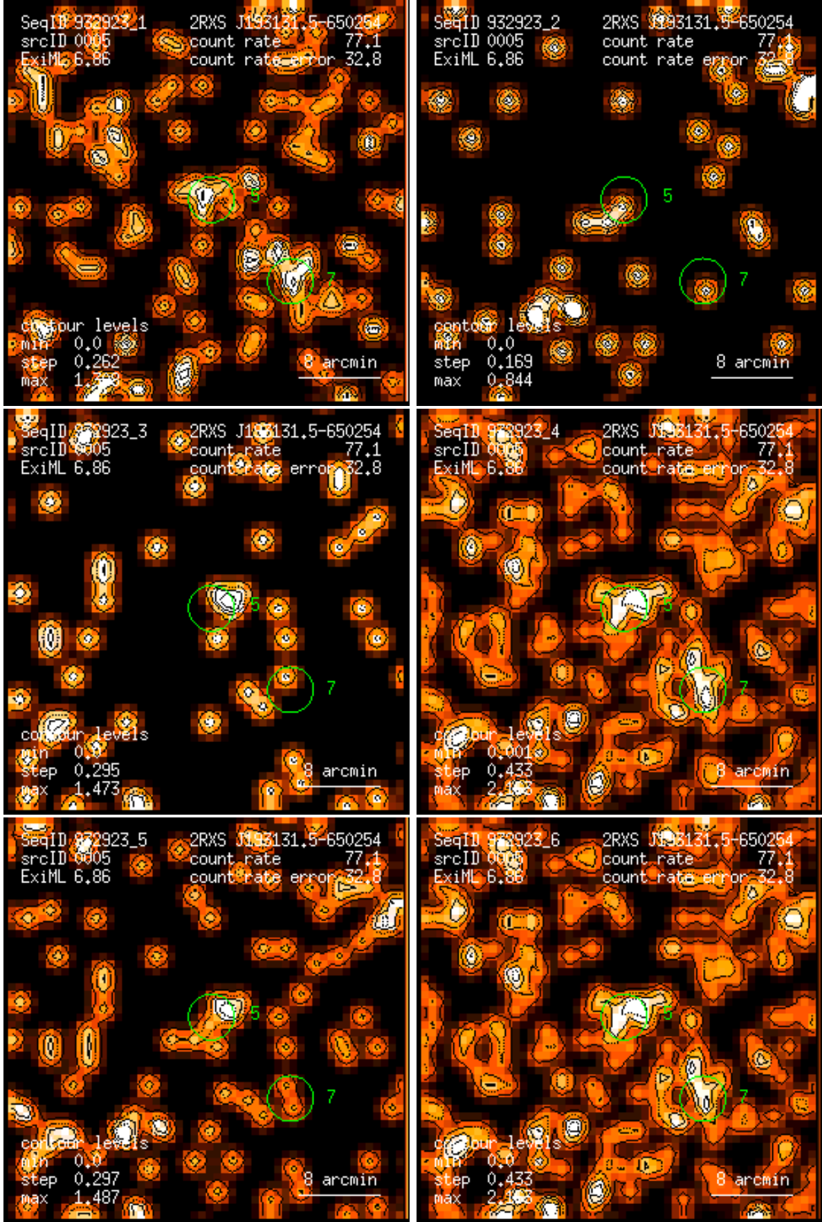
Figure 5: RASS 932923: detection 0005: band rate images, Gaussian filter: (1) PSPC channels 11 – 41, (2) 52 – 90, (3) 91 – 201, (4) 11 – 235, (5) 52 – 201, (6) 11 – 201. Broad band rates in counts/ks. Band rate contour levels in counts/ks/arcmin 2 .
