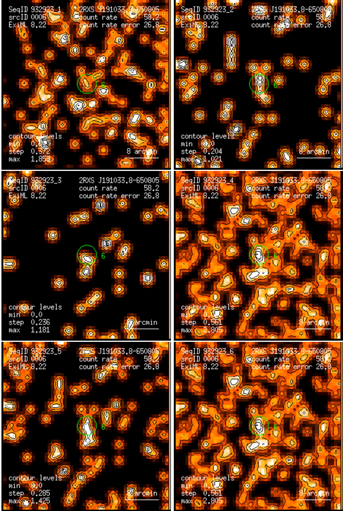
Figure 6: RASS 932923: detection 0006: band rate images, Gaussian filter: (1) PSPC channels 11 – 41, (2) 52 – 90, (3) 91 – 201, (4) 11 – 235, (5) 52 – 201, (6) 11 – 201. Broad band rates in counts/ks. Band rate contour levels in counts/ks/arcmin 2 .
