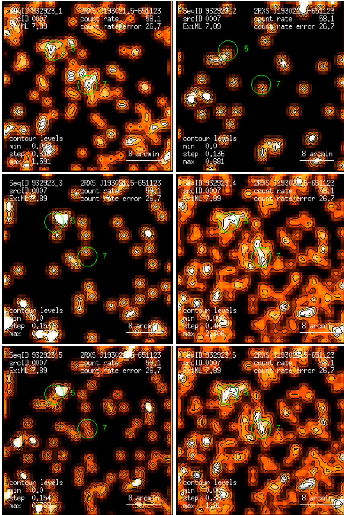
Figure 7: RASS 932923: detection 0007: band rate images, Gaussian filter: (1) PSPC channels 11 – 41, (2) 52 – 90, (3) 91 – 201, (4) 11 – 235, (5) 52 – 201, (6) 11 – 201. Broad band rates in counts/ks. Band rate contour levels in counts/ks/arcmin 2 .
