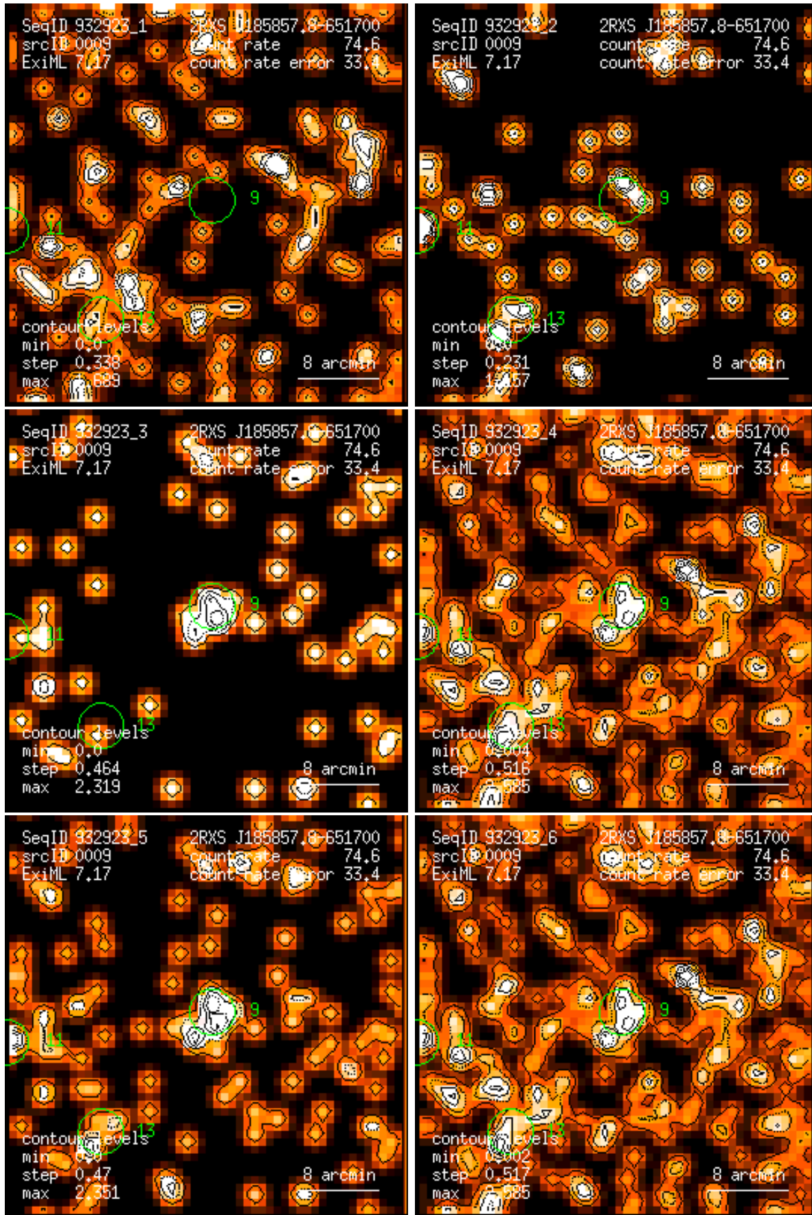
Figure 9: RASS 932923: detection 0009: band rate images, Gaussian filter: (1) PSPC channels 11 – 41, (2) 52 – 90, (3) 91 – 201, (4) 11 – 235, (5) 52 – 201, (6) 11 – 201. Broad band rates in counts/ks. Band rate contour levels in counts/ks/arcmin 2 .
