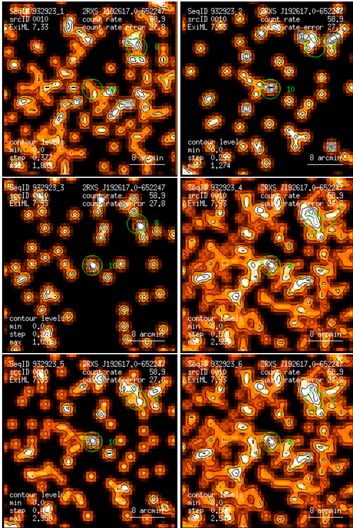
Figure 10: RASS 932923: detection 0010: band rate images, Gaussian filter: (1) PSPC channels 11 – 41, (2) 52 – 90, (3) 91 – 201, (4) 11 – 235, (5) 52 – 201, (6) 11 – 201. Broad band rates in counts/ks. Band rate contour levels in counts/ks/arcmin 2 .
