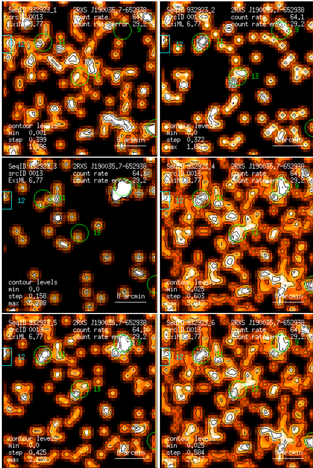
Figure 13: RASS 932923: detection 0013: band rate images, Gaussian filter: (1) PSPC channels 11 – 41, (2) 52 – 90, (3) 91 – 201, (4) 11 – 235, (5) 52 – 201, (6) 11 – 201. Broad band rates in counts/ks. Band rate contour levels in counts/ks/arcmin 2 .
