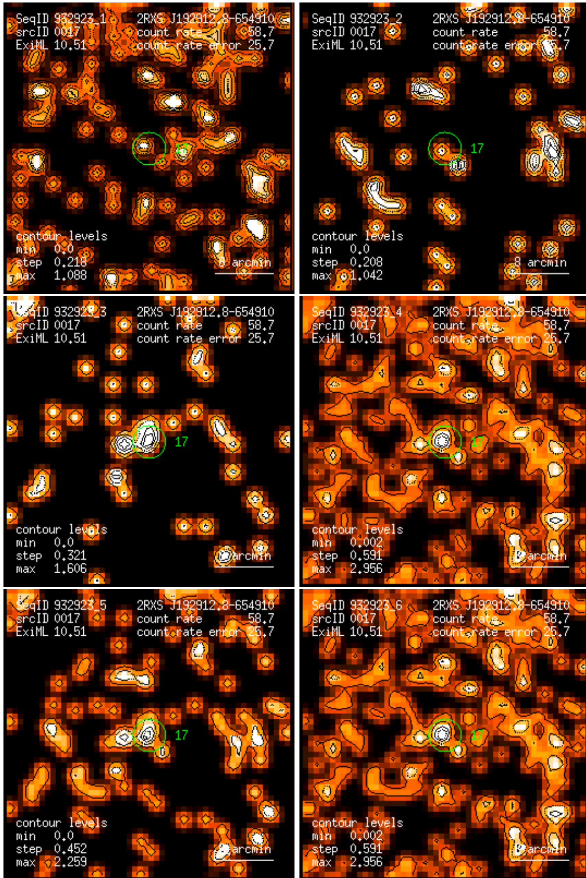
Figure 17: RASS 932923: detection 0017: band rate images, Gaussian filter: (1) PSPC channels 11 – 41, (2) 52 – 90, (3) 91 – 201, (4) 11 – 235, (5) 52 – 201, (6) 11 – 201. Broad band rates in counts/ks. Band rate contour levels in counts/ks/arcmin 2 .
