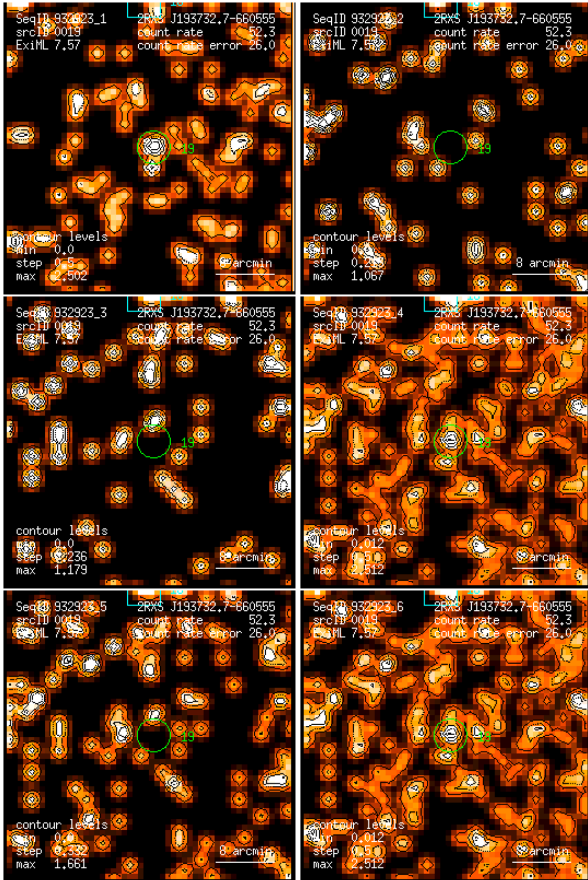
Figure 19: RASS 932923: detection 0019: band rate images, Gaussian filter: (1) PSPC channels 11 – 41, (2) 52 – 90, (3) 91 – 201, (4) 11 – 235, (5) 52 – 201, (6) 11 – 201. Broad band rates in counts/ks. Band rate contour levels in counts/ks/arcmin 2 .
