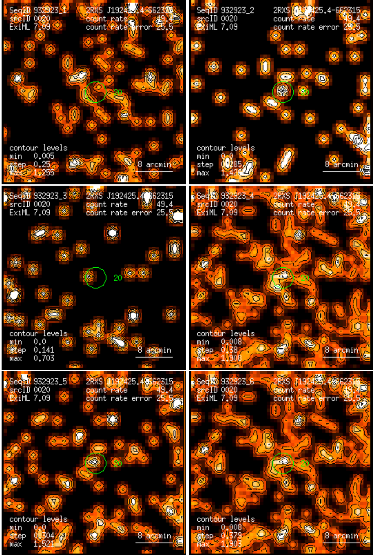
Figure 20: RASS 932923: detection 0020: band rate images, Gaussian filter: (1) PSPC channels 11 – 41, (2) 52 – 90, (3) 91 – 201, (4) 11 – 235, (5) 52 – 201, (6) 11 – 201. Broad band rates in counts/ks. Band rate contour levels in counts/ks/arcmin 2 .
