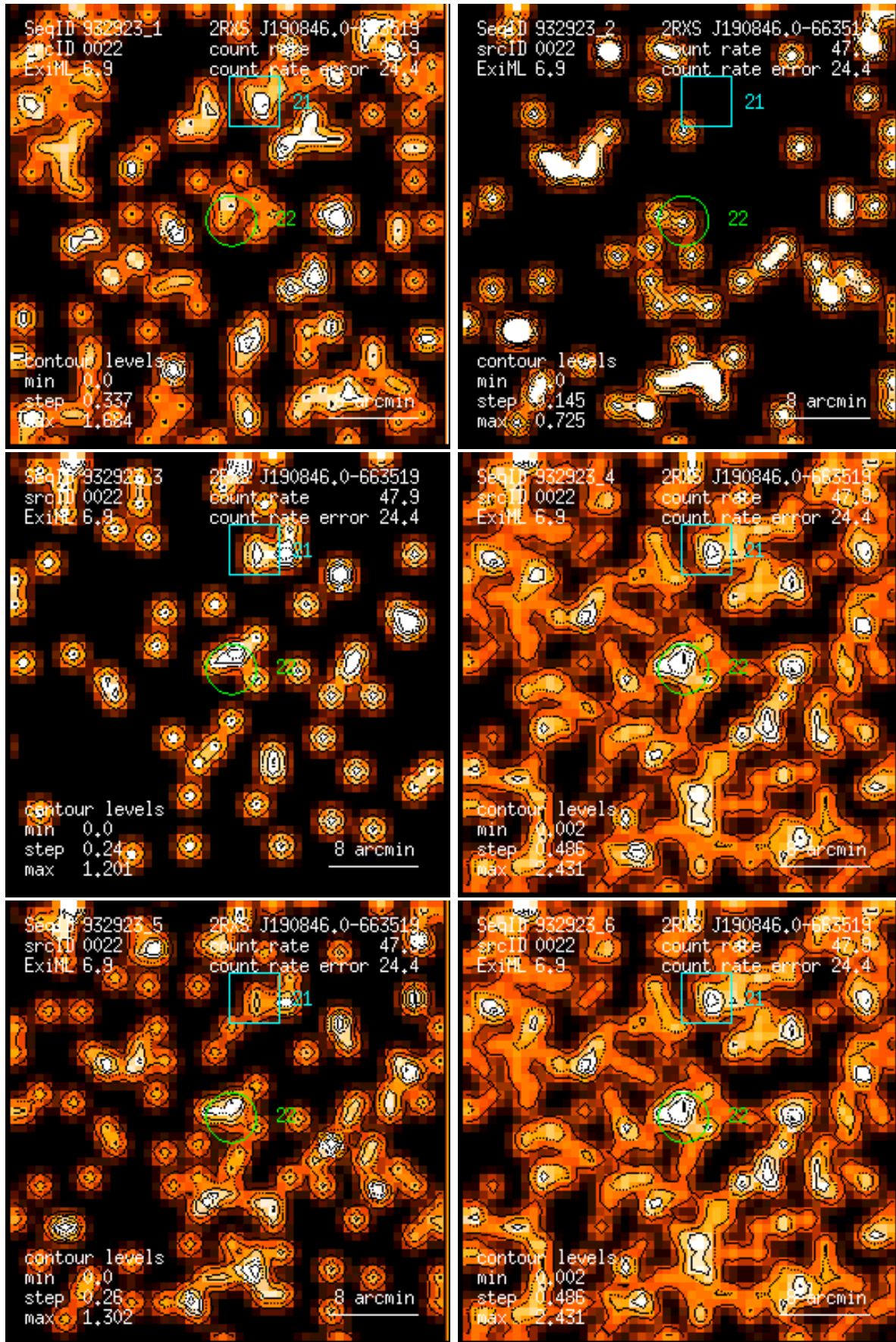
Figure 22: RASS 932923: detection 0022: band rate images, Gaussian filter: (1) PSPC channels 11 – 41, (2) 52 – 90, (3) 91 – 201, (4) 11 – 235, (5) 52 – 201, (6) 11 – 201. Broad band rates in counts/ks. Band rate contour levels in counts/ks/arcmin 2 .
