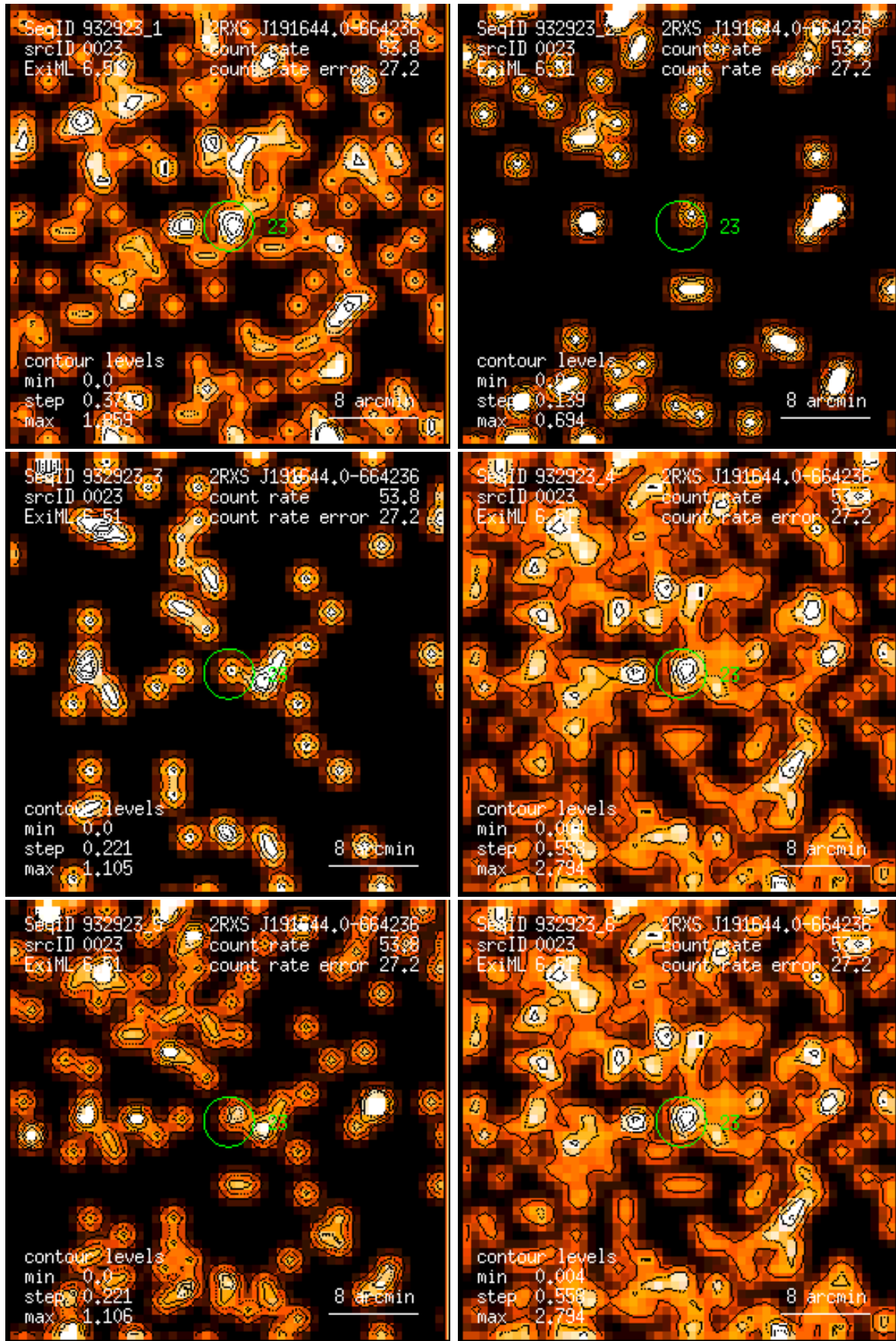
Figure 23: RASS 932923: detection 0023: band rate images, Gaussian filter: (1) PSPC channels 11 – 41, (2) 52 – 90, (3) 91 – 201, (4) 11 – 235, (5) 52 – 201, (6) 11 – 201. Broad band rates in counts/ks. Band rate contour levels in counts/ks/arcmin 2 .
