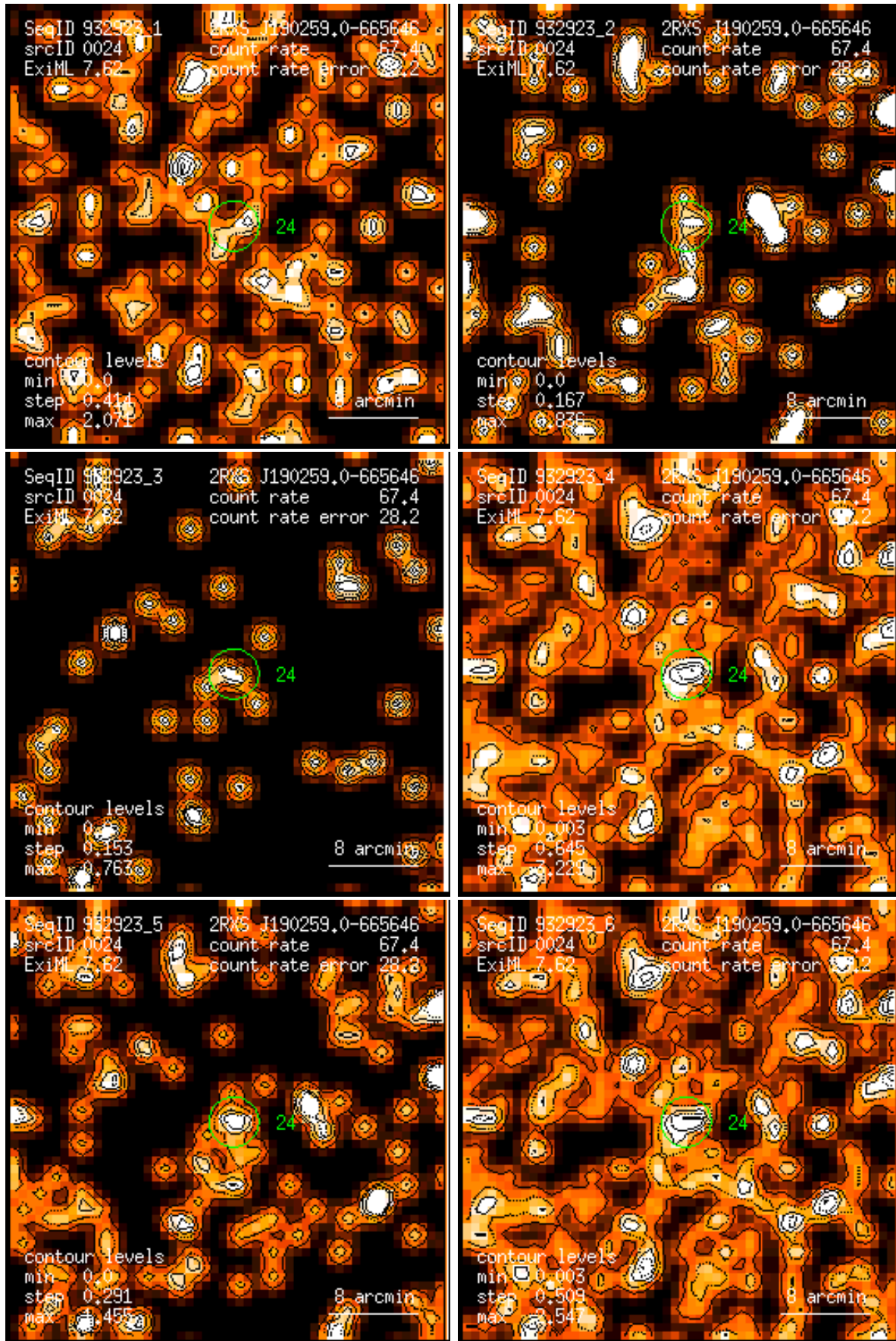
Figure 24: RASS 932923: detection 0024: band rate images, Gaussian filter: (1) PSPC channels 11 – 41, (2) 52 – 90, (3) 91 – 201, (4) 11 – 235, (5) 52 – 201, (6) 11 – 201. Broad band rates in counts/ks. Band rate contour levels in counts/ks/arcmin 2 .
