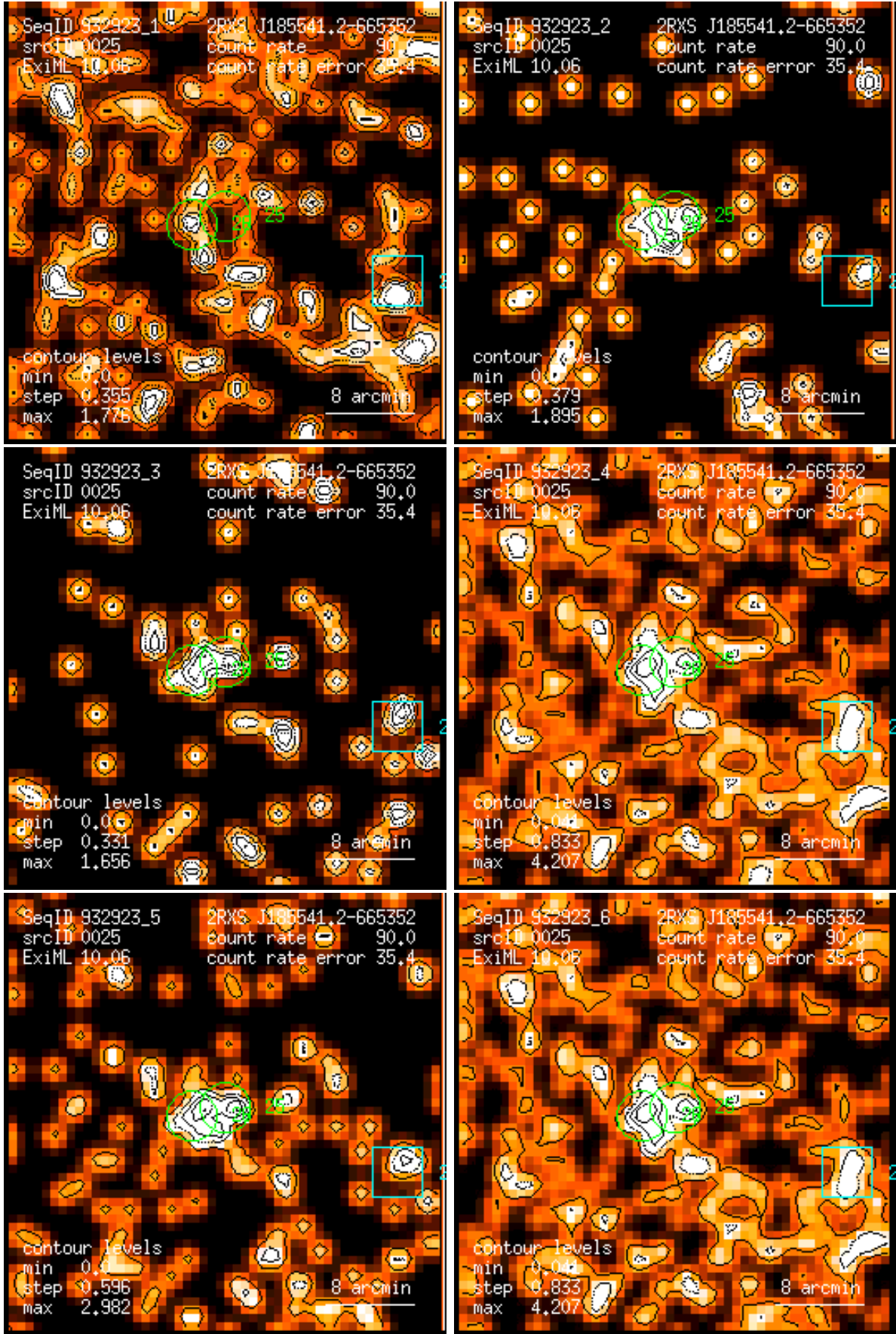
Figure 25: RASS 932923: detection 0025: band rate images, Gaussian filter: (1) PSPC channels 11 – 41, (2) 52 – 90, (3) 91 – 201, (4) 11 – 235, (5) 52 – 201, (6) 11 – 201. Broad band rates in counts/ks. Band rate contour levels in counts/ks/arcmin 2 .
