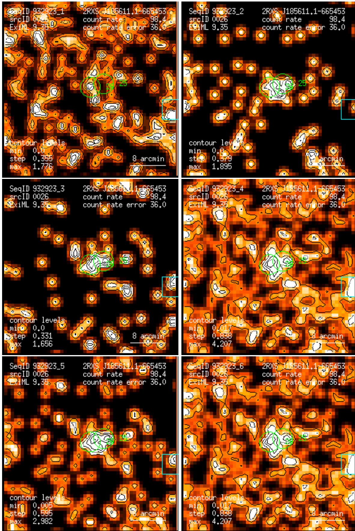
Figure 26: RASS 932923: detection 0026: band rate images, Gaussian filter: (1) PSPC channels 11 – 41, (2) 52 – 90, (3) 91 – 201, (4) 11 – 235, (5) 52 – 201, (6) 11 – 201. Broad band rates in counts/ks. Band rate contour levels in counts/ks/arcmin 2 .
