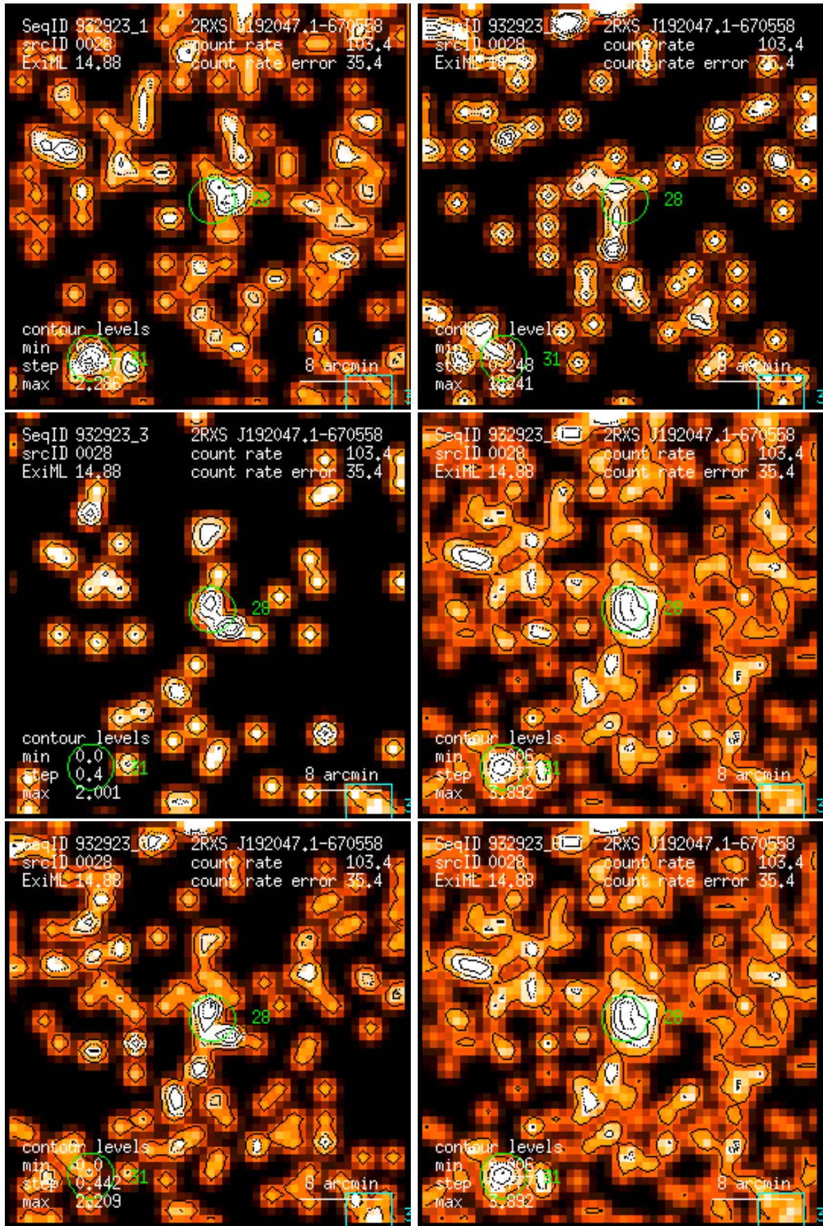
Figure 28: RASS 932923: detection 0028: band rate images, Gaussian filter: (1) PSPC channels 11 – 41, (2) 52 – 90, (3) 91 – 201, (4) 11 – 235, (5) 52 – 201, (6) 11 – 201. Broad band rates in counts/ks. Band rate contour levels in counts/ks/arcmin 2 .
