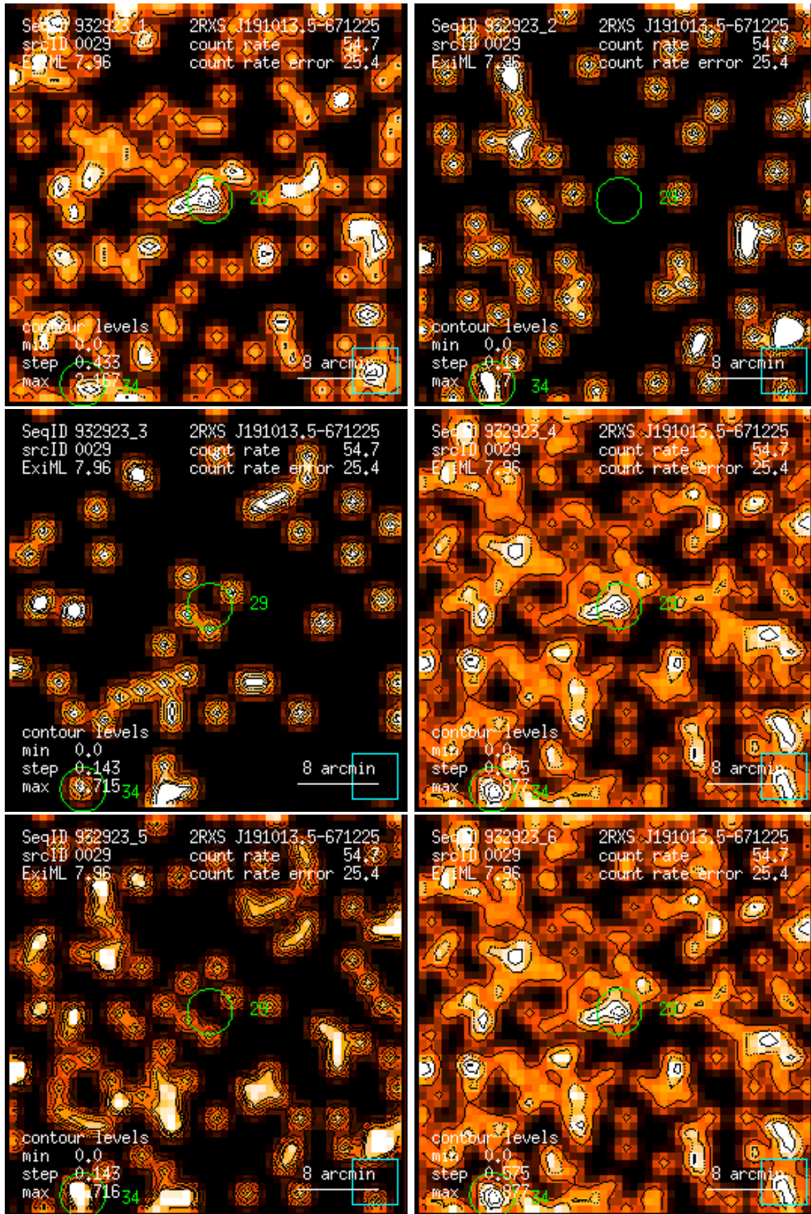
Figure 29: RASS 932923: detection 0029: band rate images, Gaussian filter: (1) PSPC channels 11 – 41, (2) 52 – 90, (3) 91 – 201, (4) 11 – 235, (5) 52 – 201, (6) 11 – 201. Broad band rates in counts/ks. Band rate contour levels in counts/ks/arcmin 2 .
