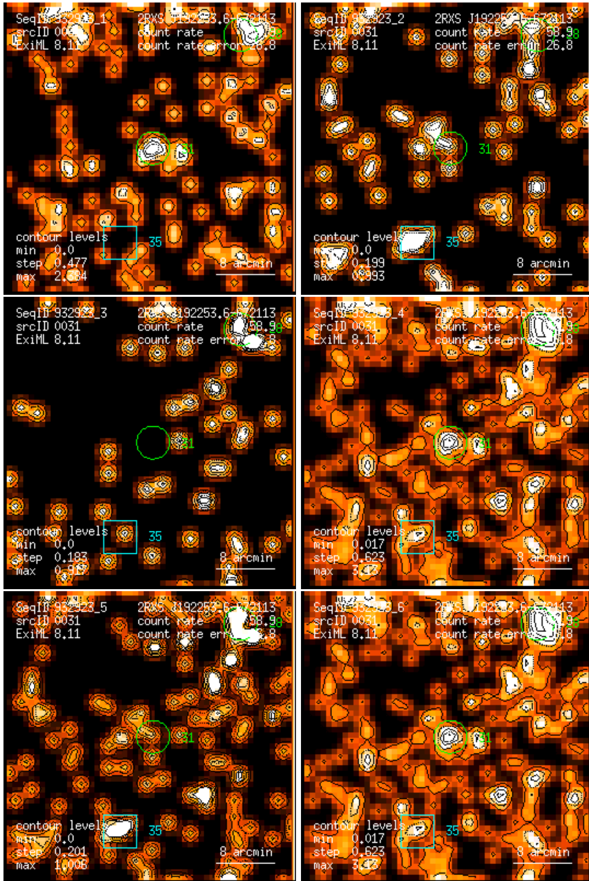
Figure 31: RASS 932923: detection 0031: band rate images, Gaussian filter: (1) PSPC channels 11 – 41, (2) 52 – 90, (3) 91 – 201, (4) 11 – 235, (5) 52 – 201, (6) 11 – 201. Broad band rates in counts/ks. Band rate contour levels in counts/ks/arcmin 2 .
