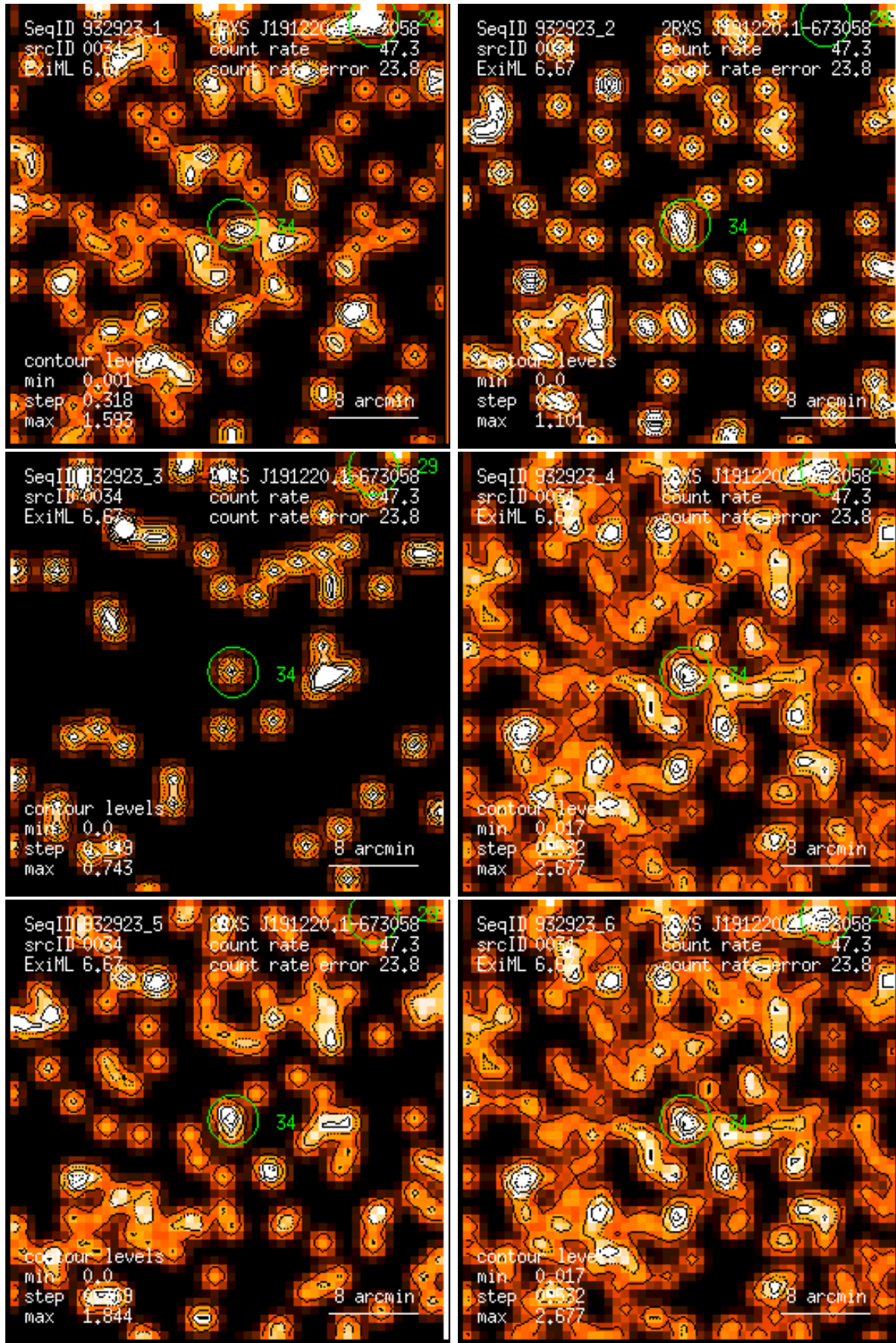
Figure 34: RASS 932923: detection 0034: band rate images, Gaussian filter: (1) PSPC channels 11 – 41, (2) 52 – 90, (3) 91 – 201, (4) 11 – 235, (5) 52 – 201, (6) 11 – 201. Broad band rates in counts/ks. Band rate contour levels in counts/ks/arcmin 2 .
