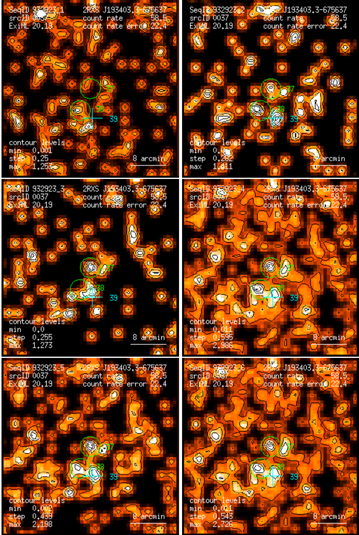
Figure 37: RASS 932923: detection 0037: band rate images, Gaussian filter: (1) PSPC channels 11 – 41, (2) 52 – 90, (3) 91 – 201, (4) 11 – 235, (5) 52 – 201, (6) 11 – 201. Broad band rates in counts/ks. Band rate contour levels in counts/ks/arcmin 2 .
