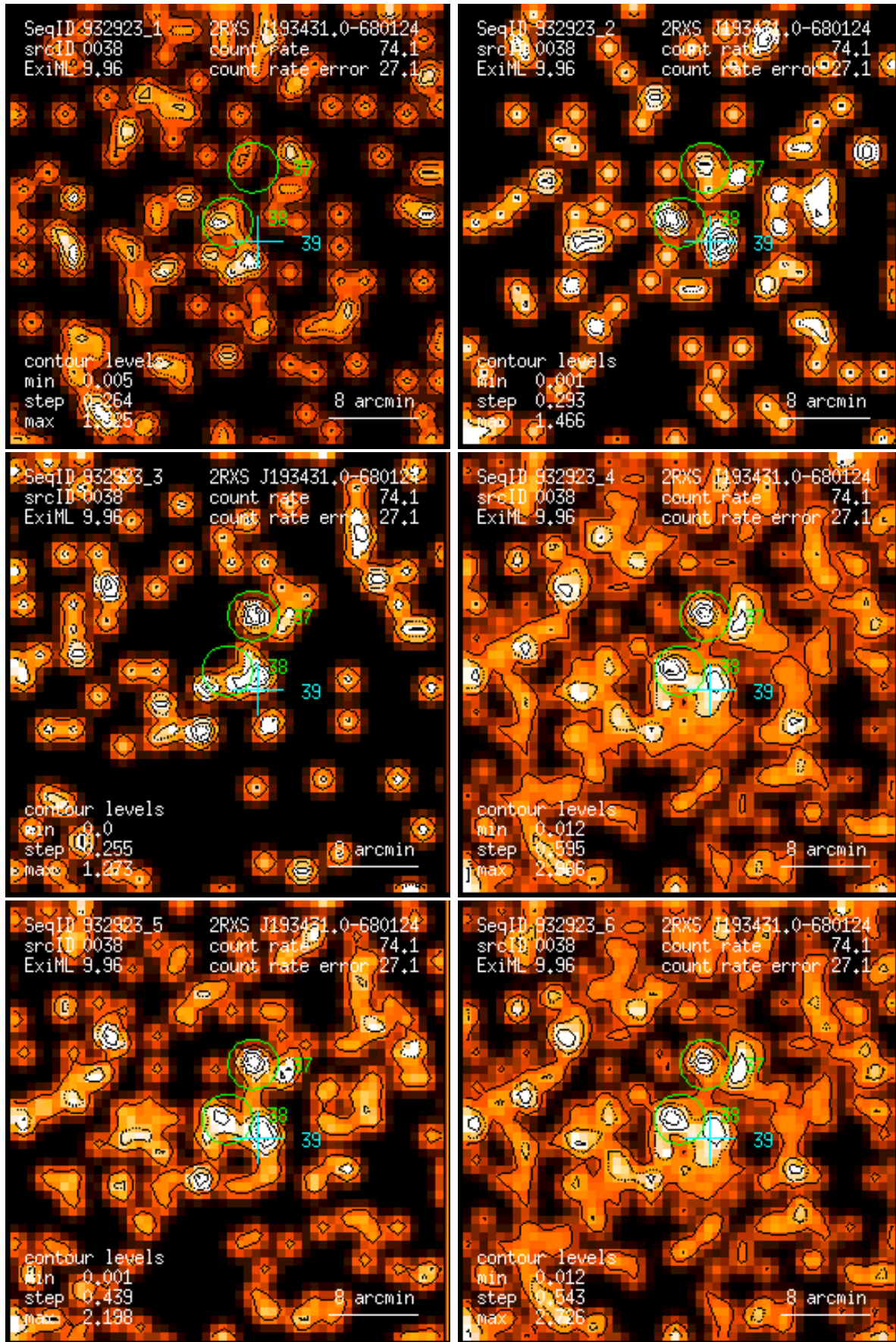
Figure 38: RASS 932923: detection 0038: band rate images, Gaussian filter: (1) PSPC channels 11 – 41, (2) 52 – 90, (3) 91 – 201, (4) 11 – 235, (5) 52 – 201, (6) 11 – 201. Broad band rates in counts/ks. Band rate contour levels in counts/ks/arcmin 2 .
