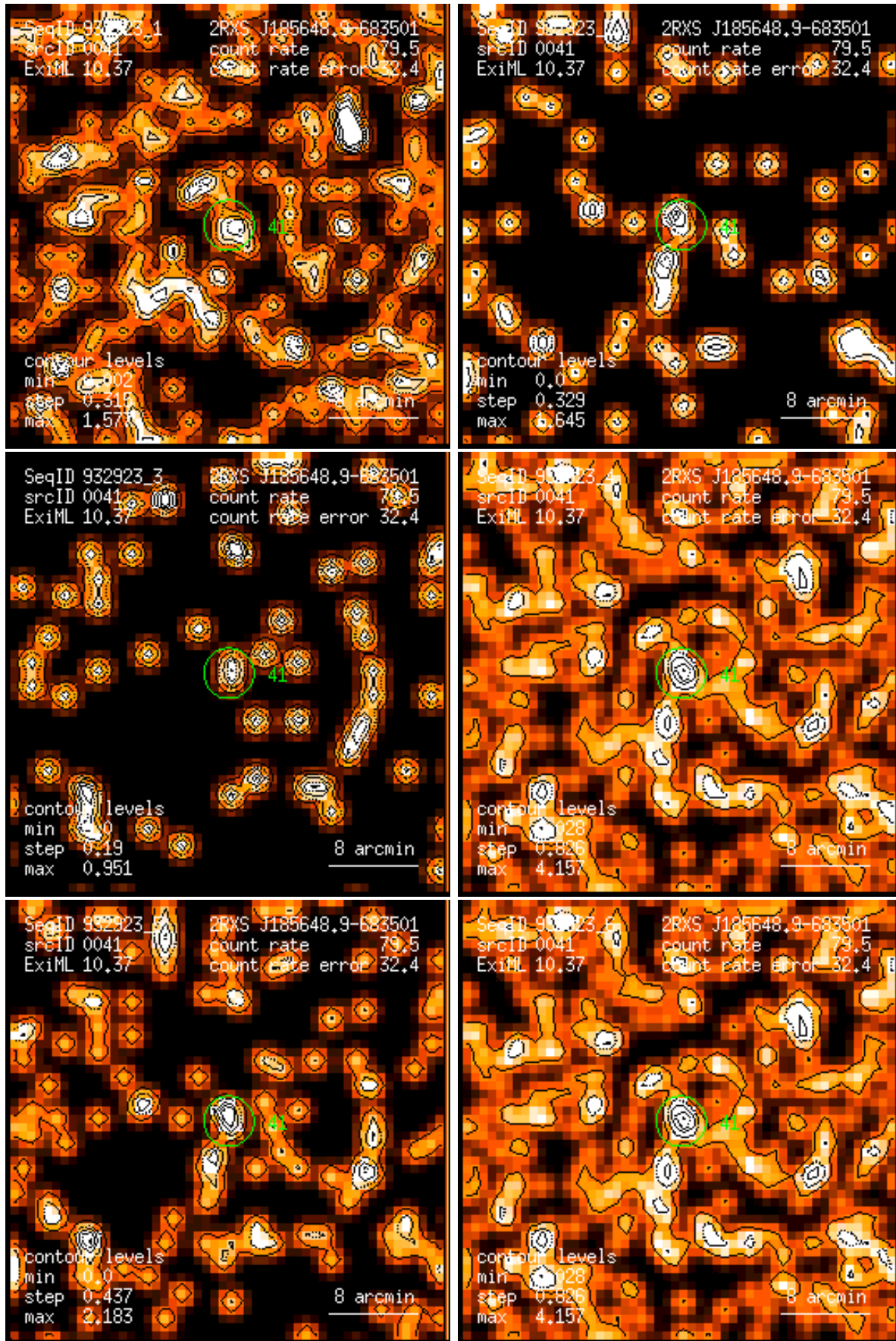
Figure 41: RASS 932923: detection 0041: band rate images, Gaussian filter: (1) PSPC channels 11 – 41, (2) 52 – 90, (3) 91 – 201, (4) 11 – 235, (5) 52 – 201, (6) 11 – 201. Broad band rates in counts/ks. Band rate contour levels in counts/ks/arcmin 2 .
