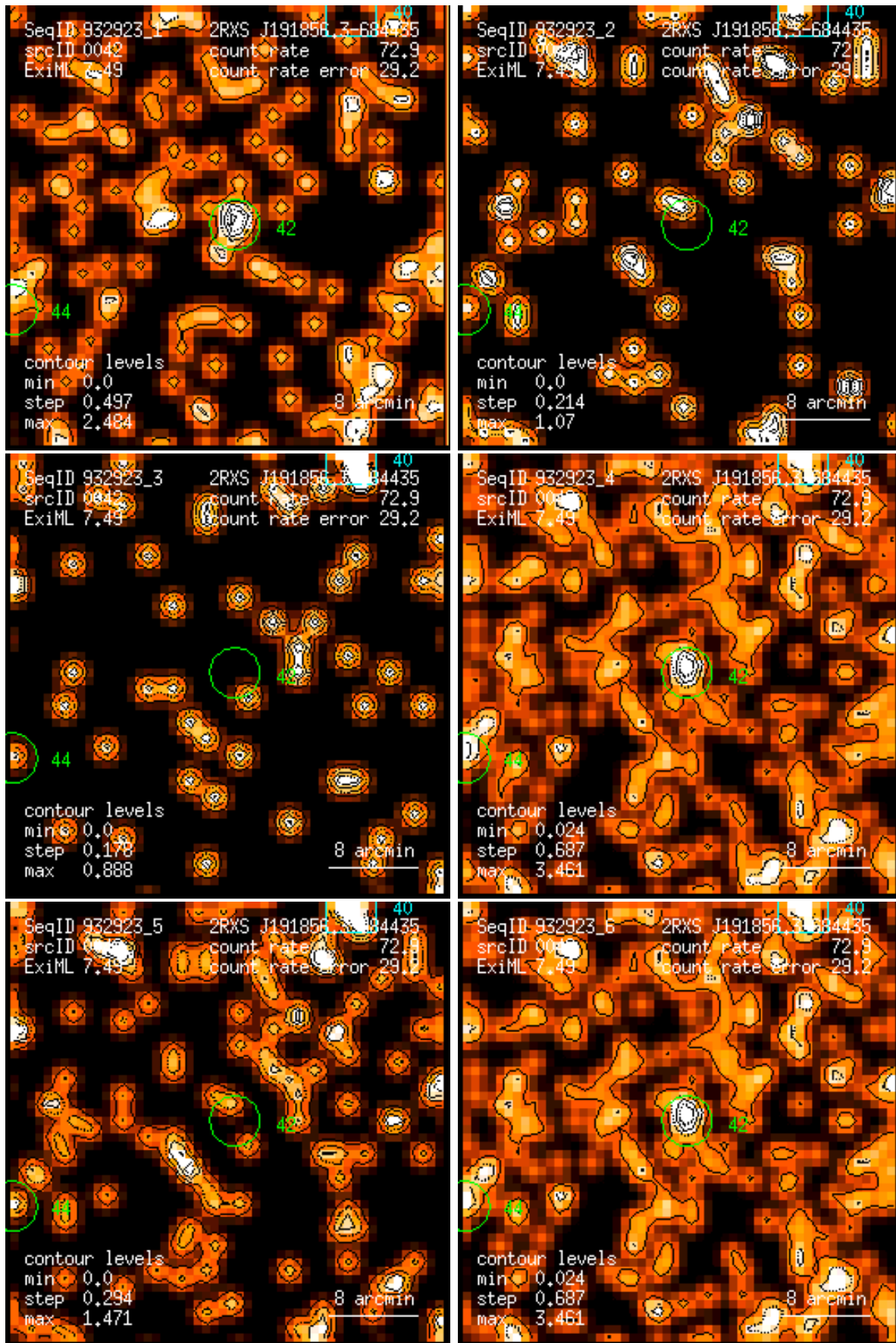
Figure 42: RASS 932923: detection 0042: band rate images, Gaussian filter: (1) PSPC channels 11 – 41, (2) 52 – 90, (3) 91 – 201, (4) 11 – 235, (5) 52 – 201, (6) 11 – 201. Broad band rates in counts/ks. Band rate contour levels in counts/ks/arcmin 2 .
