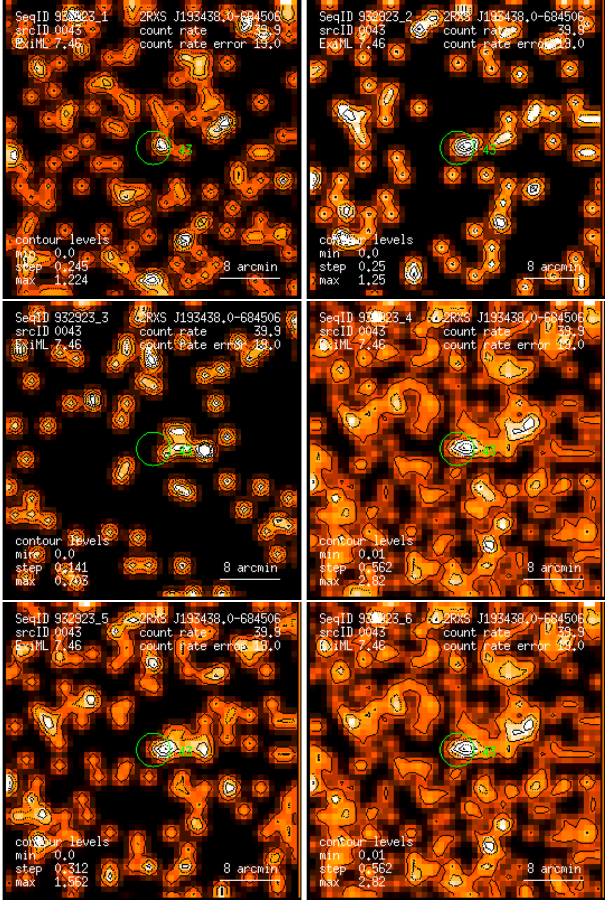
Figure 43: RASS 932923: detection 0043: band rate images, Gaussian filter: (1) PSPC channels 11 – 41, (2) 52 – 90, (3) 91 – 201, (4) 11 – 235, (5) 52 – 201, (6) 11 – 201. Broad band rates in counts/ks. Band rate contour levels in counts/ks/arcmin 2 .
