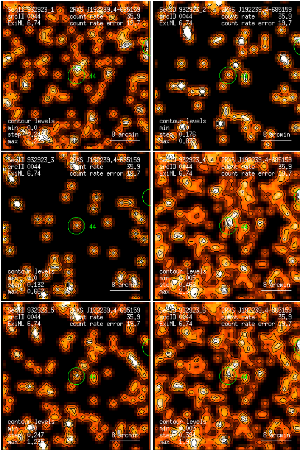
Figure 44: RASS 932923: detection 0044: band rate images, Gaussian filter: (1) PSPC channels 11 – 41, (2) 52 – 90, (3) 91 – 201, (4) 11 – 235, (5) 52 – 201, (6) 11 – 201. Broad band rates in counts/ks. Band rate contour levels in counts/ks/arcmin 2 .
