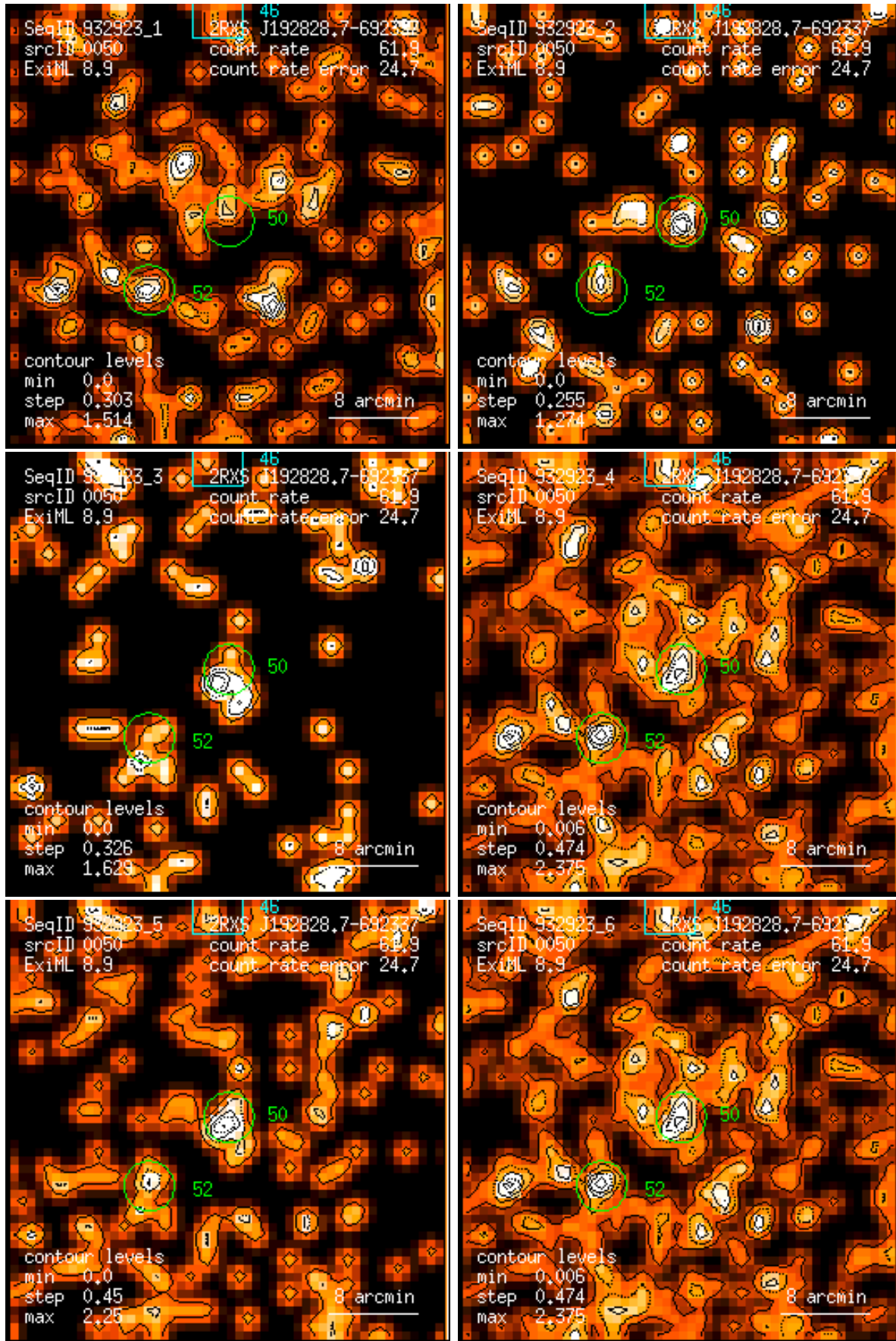
Figure 50: RASS 932923: detection 0050: band rate images, Gaussian filter: (1) PSPC channels 11 – 41, (2) 52 – 90, (3) 91 – 201, (4) 11 – 235, (5) 52 – 201, (6) 11 – 201. Broad band rates in counts/ks. Band rate contour levels in counts/ks/arcmin 2 .
